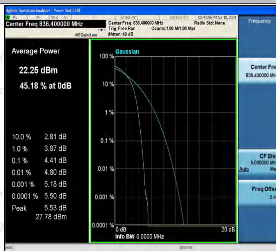
Band5-4182-5-PASS
