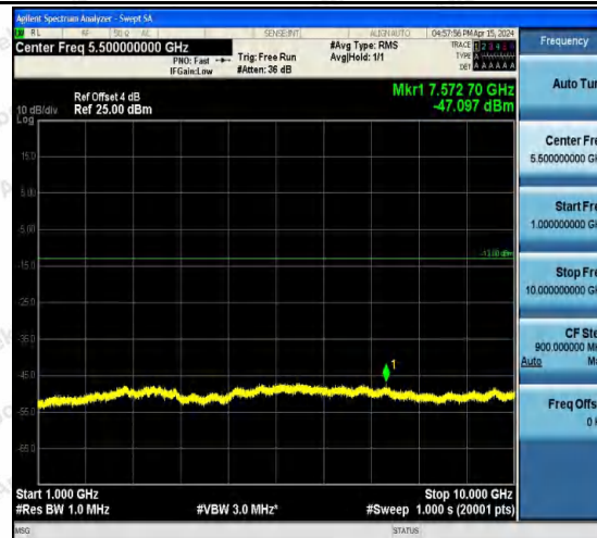
Band5-4132-4-1000~10000MHz-PASS
