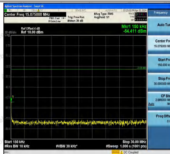
Band5-4182-2-0.15~30MHz-PASS
