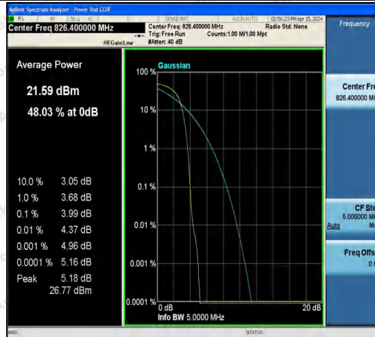
Band5-4132-4-PASS
