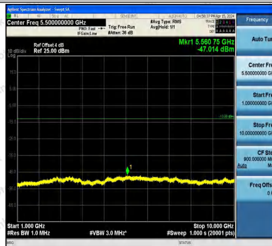
Band5-4182-4-1000~10000MHz-PASS
