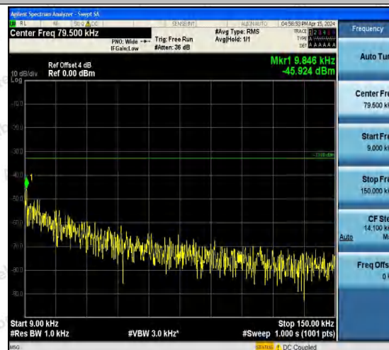
Band5-4233-4-0.009~0.15MHz-PASS
