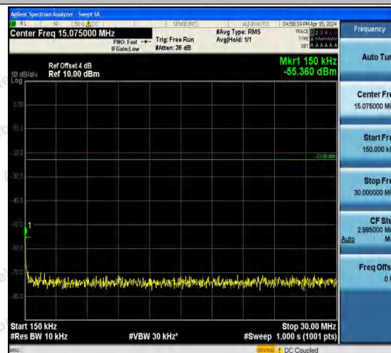
Band5-4182-4-0.15~30MHz-PASS
