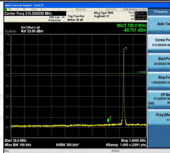
Band5-4182-4-30~1000MHz-PASS
