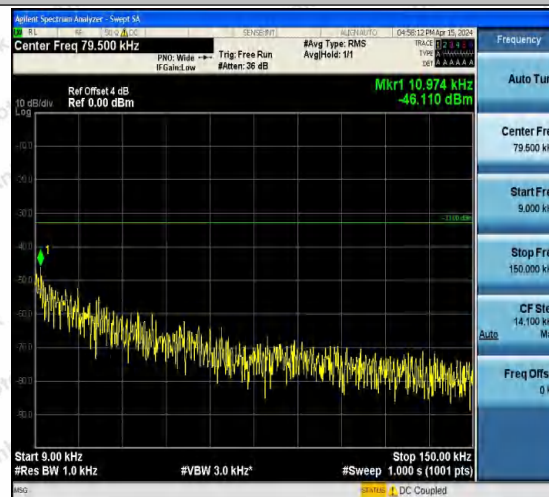
Band5-4182-4-0.009~0.15MHz-PASS
