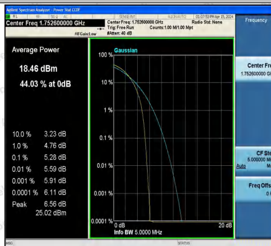
Band4-1513-3-PASS
