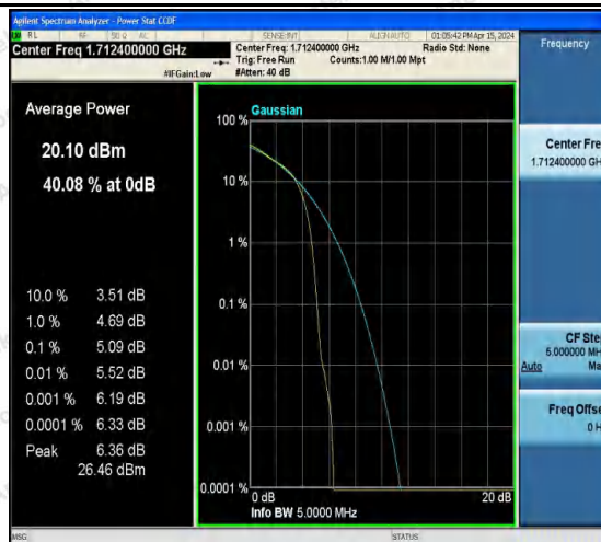
Band4-1312-2-PASS
