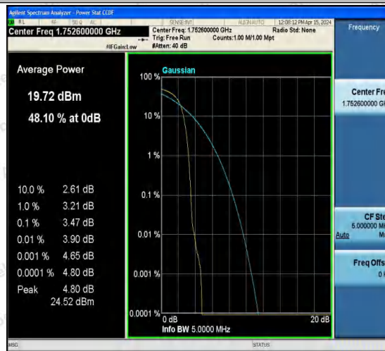
Band4-1513-2-PASS
