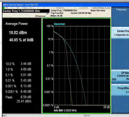
Band4-1513-2-PASS
