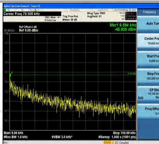
Band4-1413-3-0.009~0.15MHz-PASS
