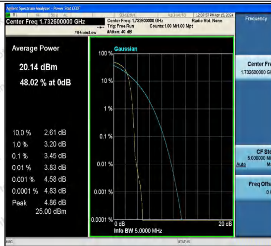
Band4-1413-2-PASS
