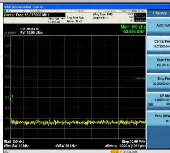
Band4-1413-3-0.15~30MHz-PASS
