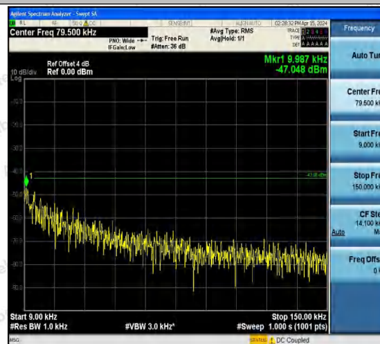
Band4-1513-3-0.009~0.15MHz-PASS
