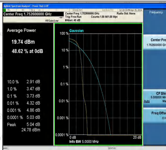
Band4-1513-4-PASS
