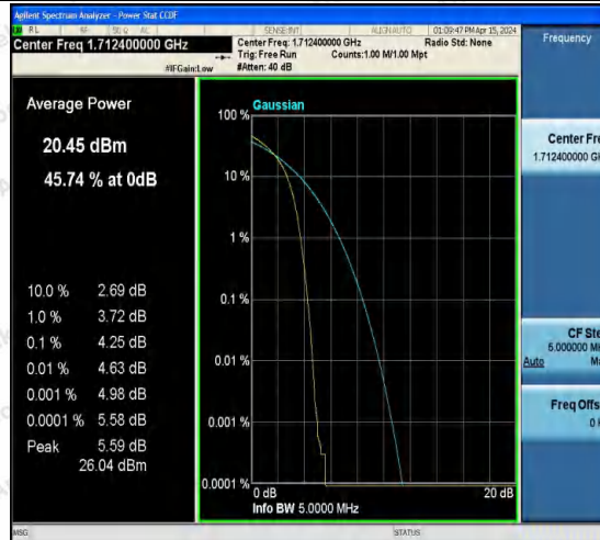
Band4-1312-5-PASS
