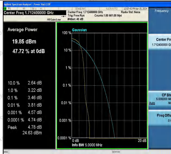
Band4-1312-2-PASS
