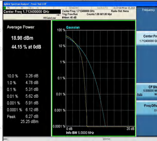
Band4-1312-3-PASS
