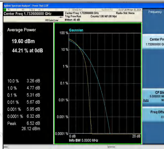
Band4-1413-3-PASS
