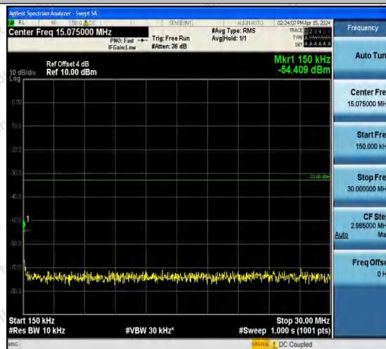
Band4-1312-2-0.15~30MHz-PASS
