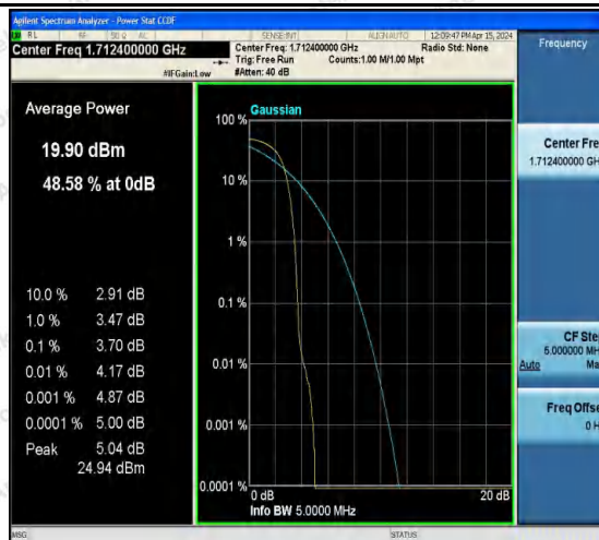
Band4-1312-4-PASS
