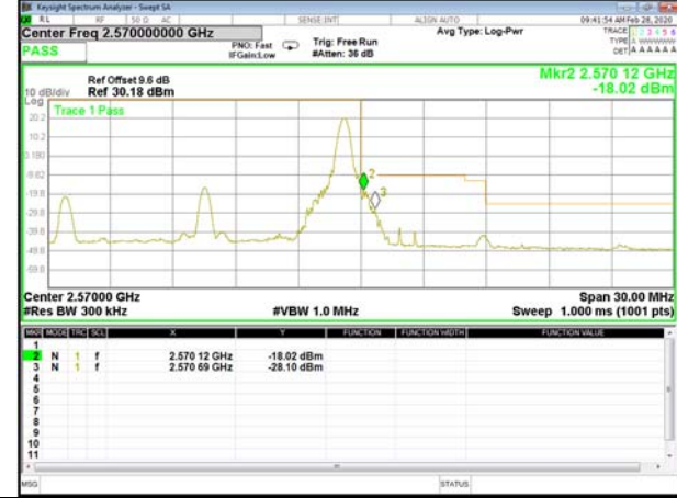
B7_QPSK_20M_Low_1-RB_Bedge
