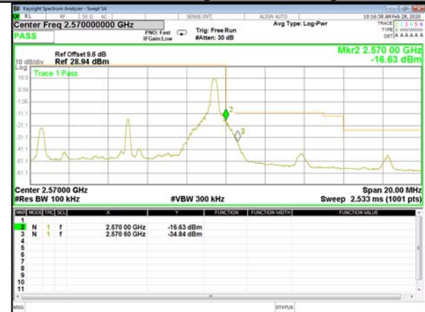
B7_QPSK_10M_Higher_Band edge_1-RB
