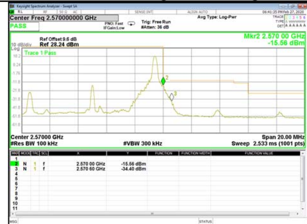
B7_Q16_10M_High_1-RB_Bedge
