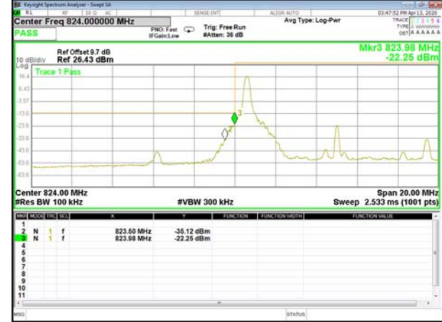
B5_QPSK_10M_High_1-RB_Bedge
