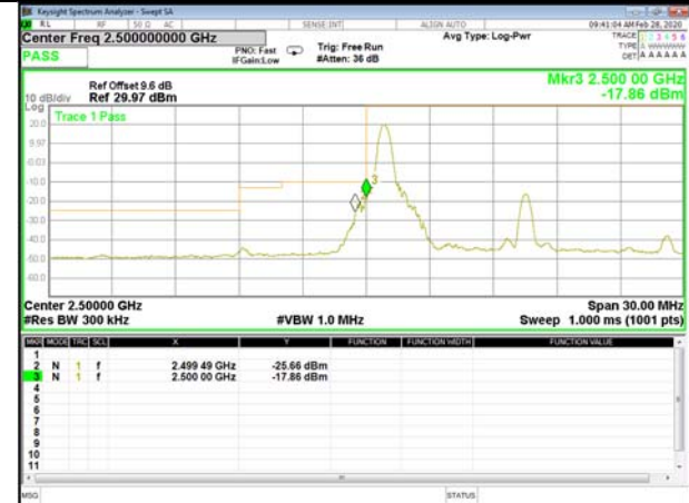
B7_Q16_15M_Low_1-RB_Bedge
