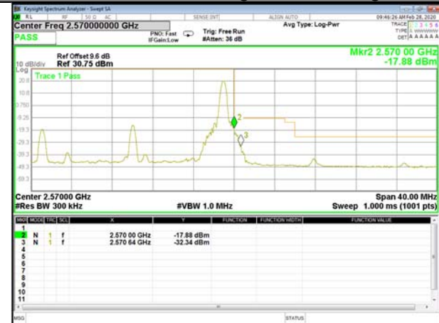
B7_QPSK_20M_High_1-RB_Bedge
