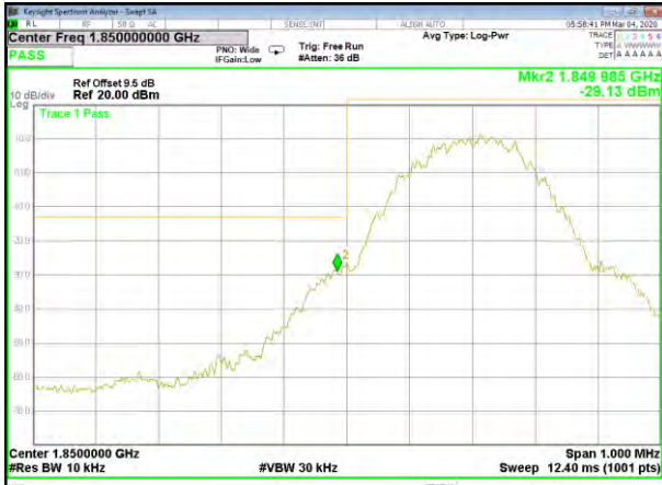
GSM 1900 Lower Band edge
