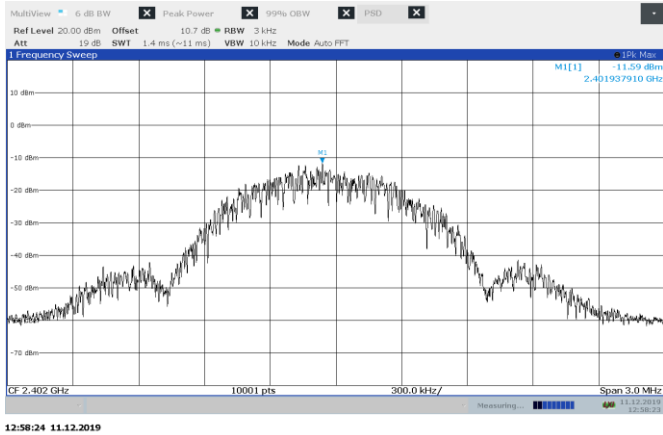
Figure 8.7-1: PSD, low channel
