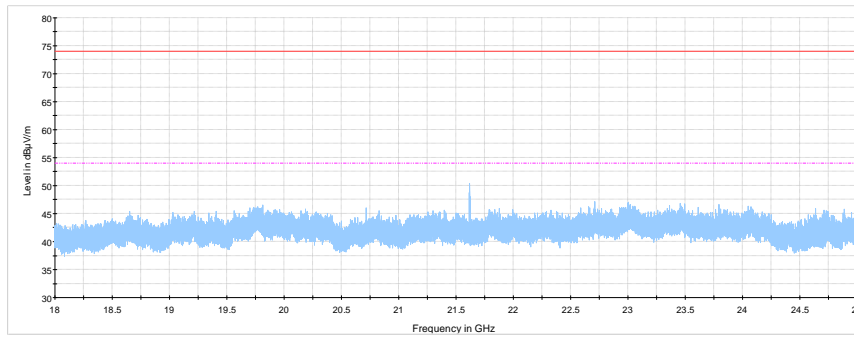
NEX389263 18-25 GHz BLE low channel Preview Result 1-PK+ FCC Part 15 and ICES-003 Limit - Class B (Peak) above 1 GHz, 3 m FCC Part 15 and ICES-003 Limit - Class B (Quasi-Peak and Average), 3 m
