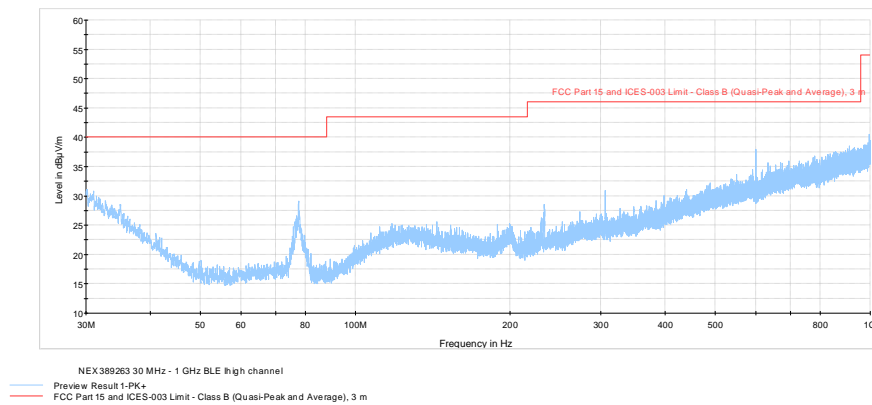
Figure 8.6-7: Radiated spurious emissions 30 MHz – 1 GHz, BLE High channel
