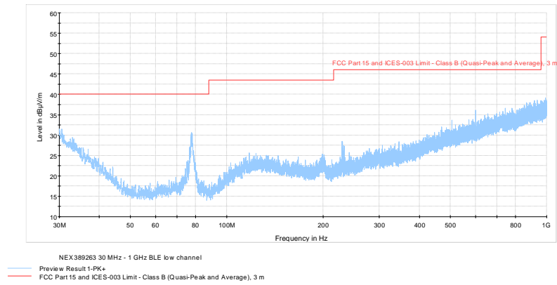
Figure 8.6-5: Radiated spurious emissions 30 MHz – 1 GHz, BLE Low channel
