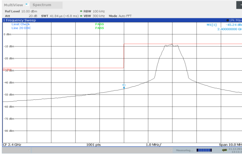
Figure 8.6-14: Conducted band edge emissions for BLE Low channel
