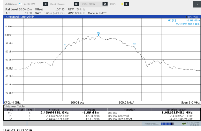
Figure 8.4-5: 99% Occupied Bandwidth, mid channel
