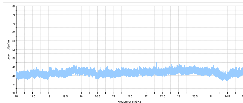
NEX389263 18-25 GHz BLE High channel Preview Result 1-PK+ FCC Part 15 and ICES-003 Limit - Class B (Peak) above 1 GHz, 3 m FCC Part 15 and ICES-003 Limit - Class B (Quasi-Peak and Average), 3 m
