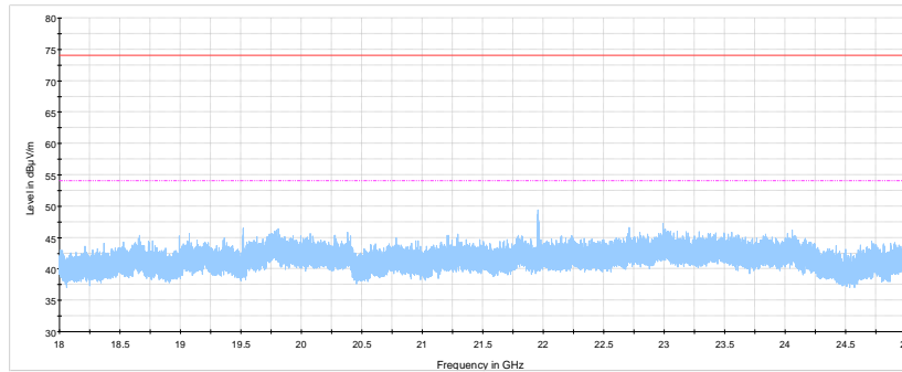
NEX389263 18-25 GHz BLE Mid channel Preview Result 1-PK+ FCC Part 15 and ICES-003 Limit - Class B (Peak) above 1 GHz, 3 m FCC Part 15 and ICES-003 Limit - Class B (Quasi-Peak and Average), 3 m
