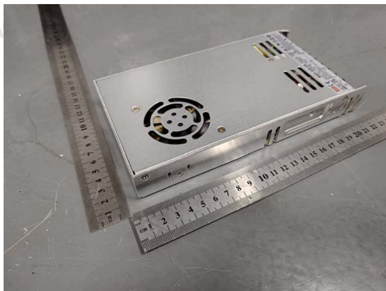
Built-in power supply: RSP-320-24
