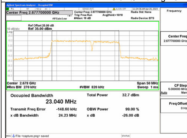
Band41C / 15MHz+10MHz / 16QAM/ High CH
