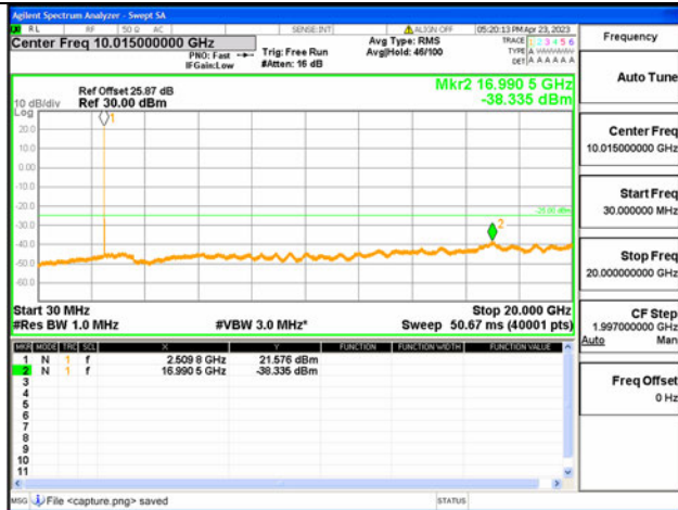
7C-30M-20G / 10+20MHz / QPSK / Low CH / #49-1#0
