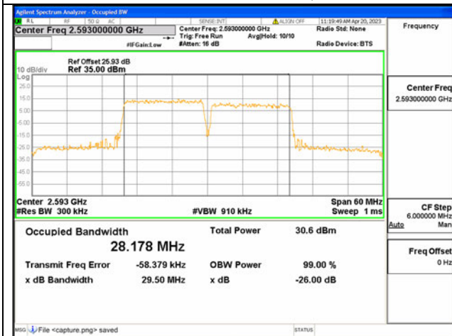
Band41C / 15MHz+15MHz / 64QAM/ Mid CH
