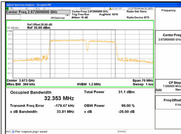
Band41C / 20MHz+15MHz / QPSK/ High CH
