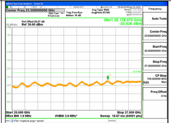
7C-20G-27G / 10+20MHz / QPSK / Low CH / #49-1#0
