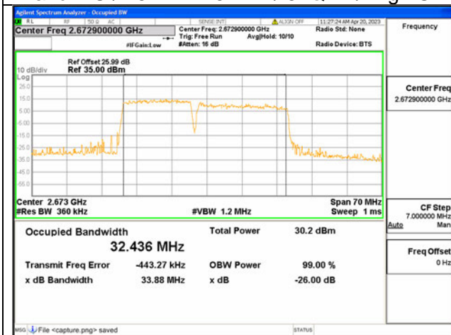
Band41C / 15MHz+20MHz / 16QAM/ High CH
