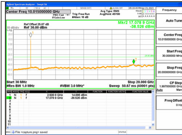
7C-30M-20G / 10+20MHz / QPSK / Low CH / #0-1#99
