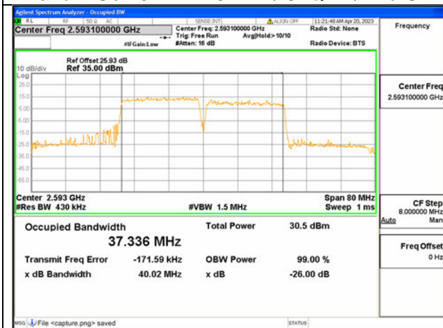
Band41C / 20MHz+20MHz / 16QAM/ Mid CH
