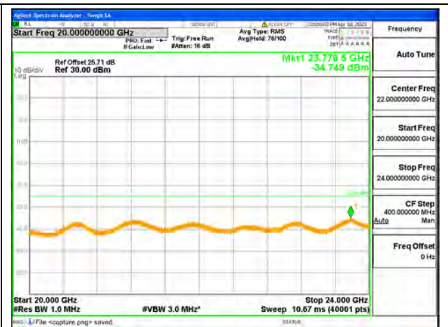
Band30-20G-24G / 5MHz / Low CH / QPSK
