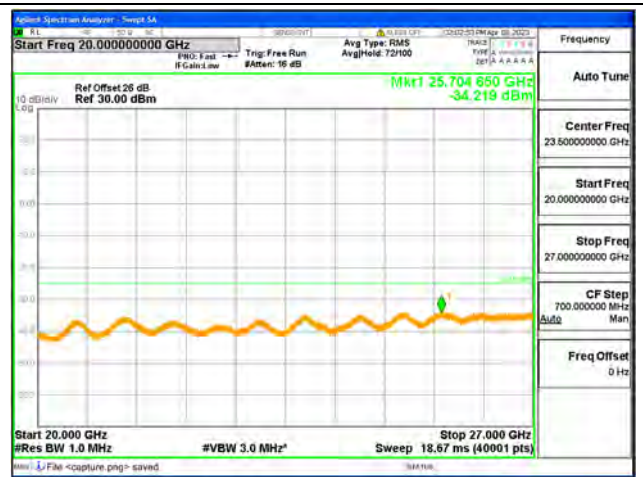
Band41-20G-27G / 15MHz / High CH / QPSK
