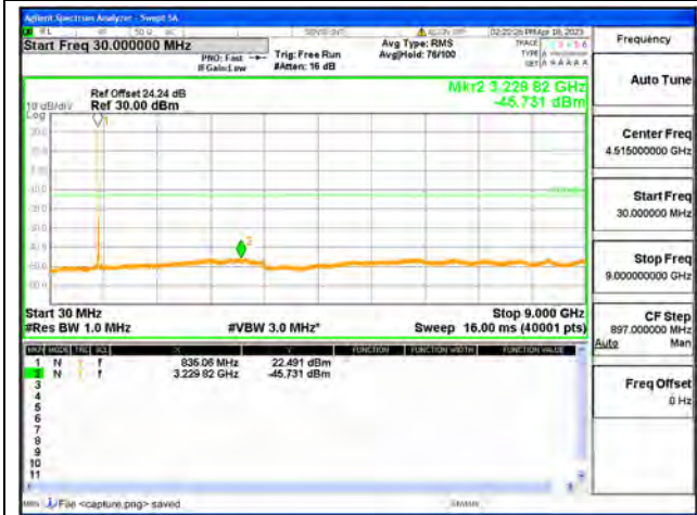
Band26 Part22 / 15MHz / High CH / QPSK
