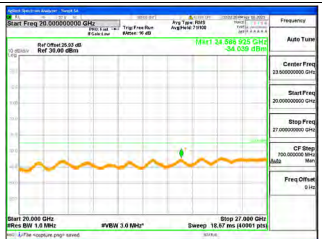
Band41-20G-27G / 15MHz / Mid CH / QPSK
