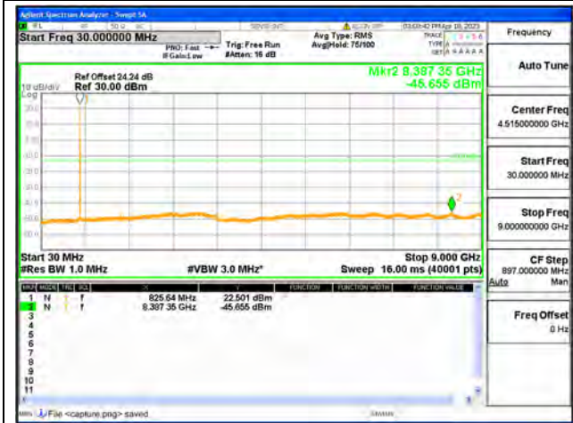
Band18 part22 / 5MHz / High CH / QPSK
