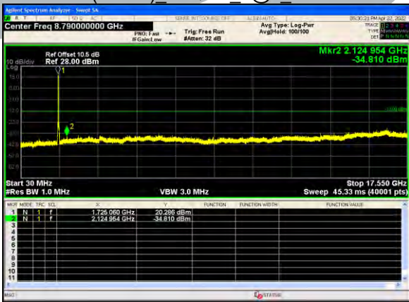
B4(20.0M) 16QAM 1@0 Middle
