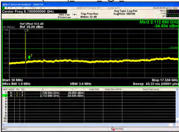
B4(20.0M) 64QAM 1@0 Lowest
