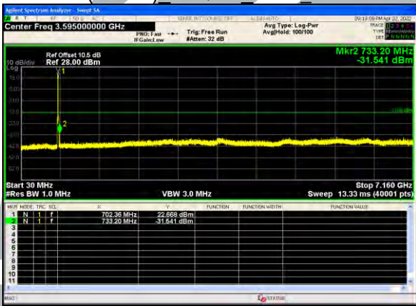
B12(10.0M) 16QAM 1RB0 Middle
