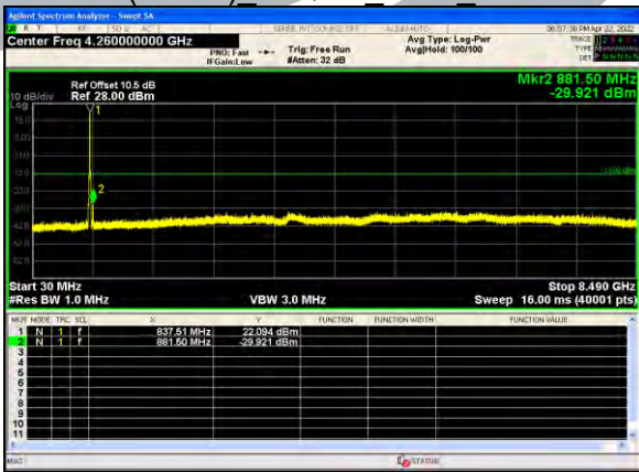
B5(10.0M) 16QAM 1RB0 Middle
