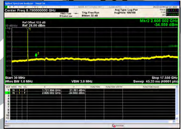
B4(15.0M) 16QAM 1@0 Middle
