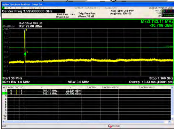
B17(10.0M) 16QAM 1@0 Middle
