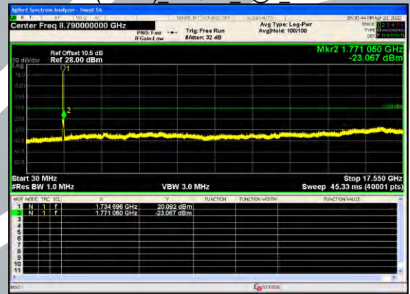
B4(20.0M) 64QAM 1@0 Middle
