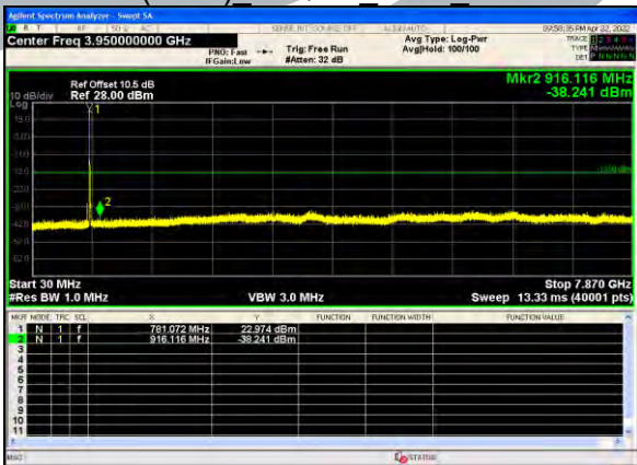
B13(5.0M) 16QAM 1RB0 Lowest
