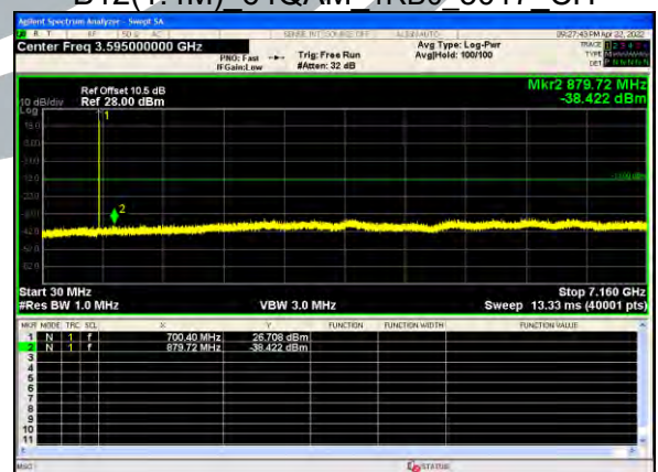
B12(1.4M) 64QAM 1RB0 5017 CH
