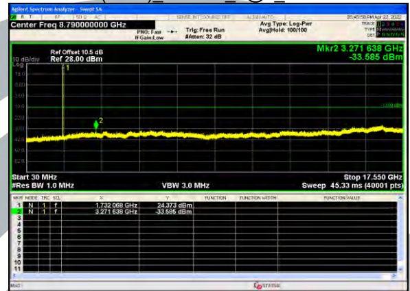
B4(3.0M) 16QAM 1@0 Highest
