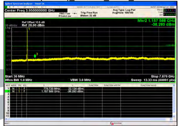
B13(5.0M) QPSK 1RB0 Lowest
