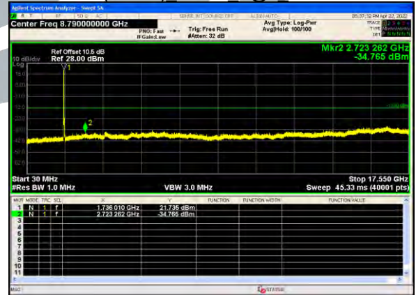
B4(10.0M) QPSK 1@0 Middle
