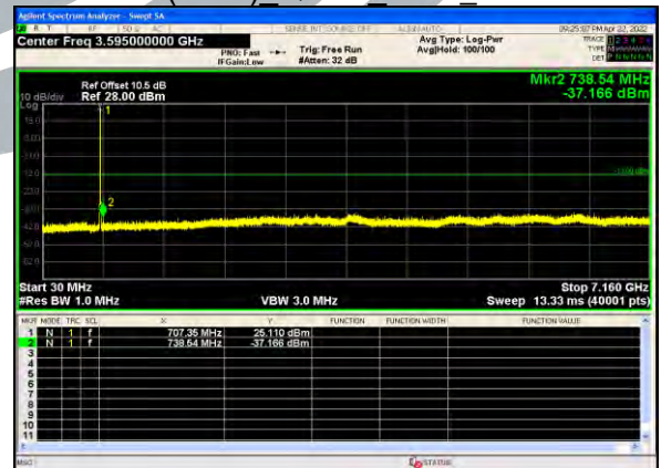
B12(3.0M) QPSK 1RB0_Middle
