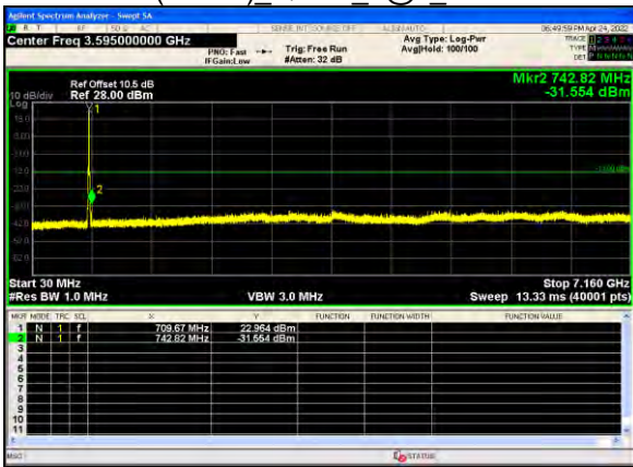
B17(10.0M) 64QAM 1@0 Lowest
