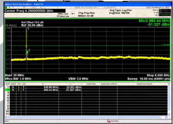
B5(10.0M) 64QAM 1RB0 Middle
