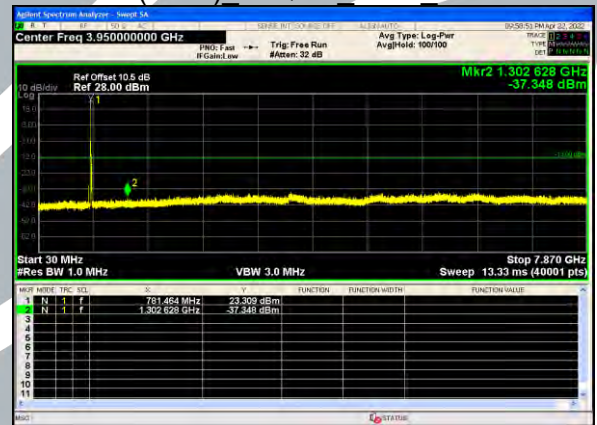
B13(5.0M) 64QAM 1RB0 Lowest
