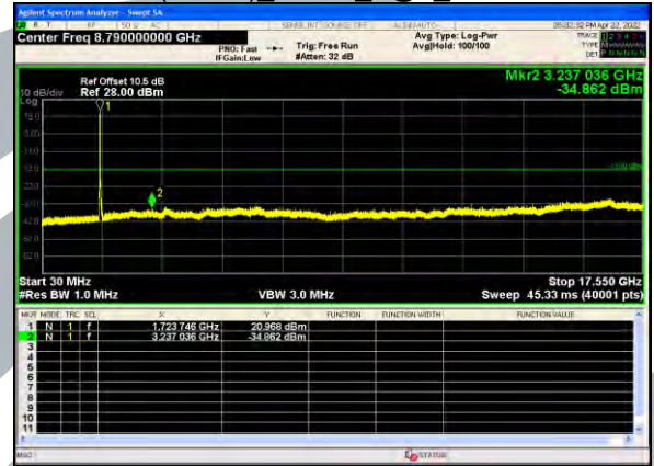
B4(15.0M) 64QAM 1@0 Lowest
