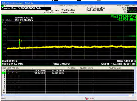
B12(10.0M) 64QAM 1RB0 Lowest
