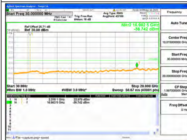
Band30-30M-20G / 5MHz / High CH / QPSK
