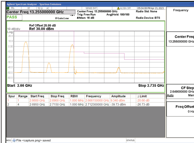
41C / 10+15MHz / High CH / QPSK / 1#0-1#74
