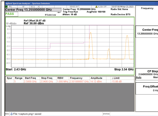
7C / 15+20MHz / Low CH / QPSK / 1#0-1#99
