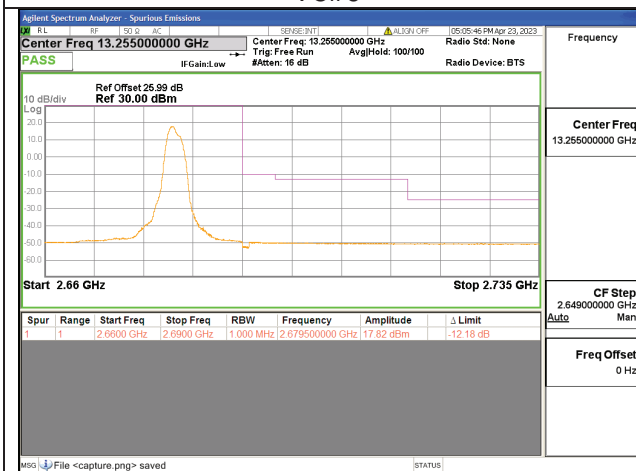
41C / 15+10MHz / High CH / QPSK / 1#74-1#0
