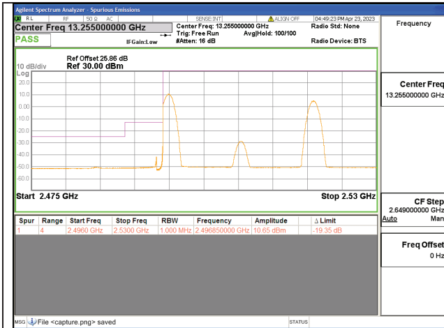
41C / 10+15MHz / Low CH / QPSK / 1#0-1#74
