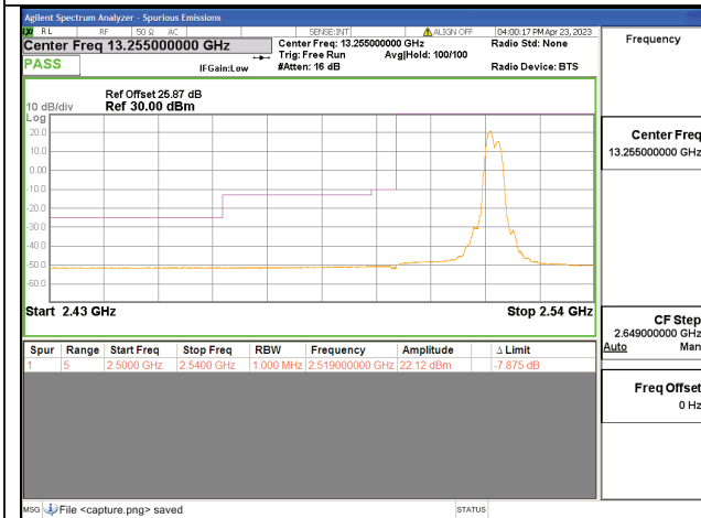
7C / 20+15MHz / Low CH / QPSK / 1#99-1#0
