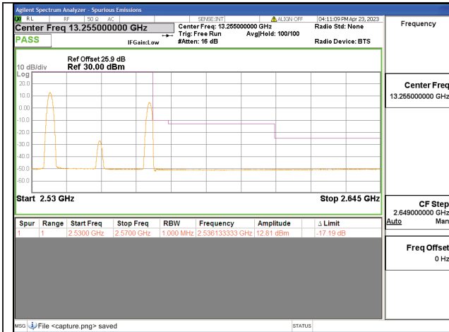
7C / 20+15MHz / High CH / QPSK / 1#0-1#74
