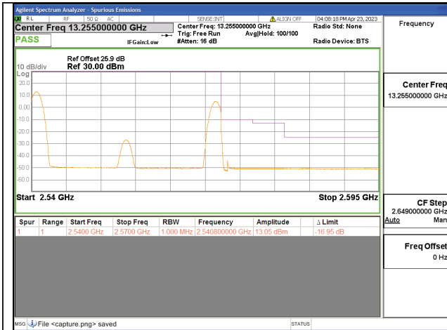
7C / 15+15MHz / High CH / QPSK / 1#0-1#74
