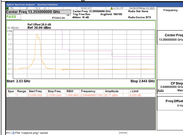
7C / 15+20MHz / High CH / QPSK / 1#74-1#0
