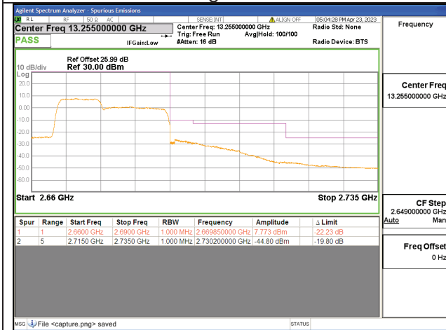
41C / 10+15MHz / High CH / QPSK / 50#0-75#0
