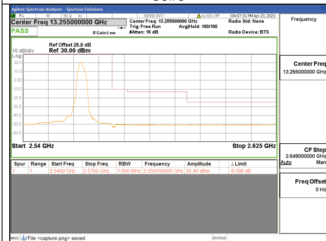
7C / 15+10MHz / High CH / QPSK / 1#74-1#0
