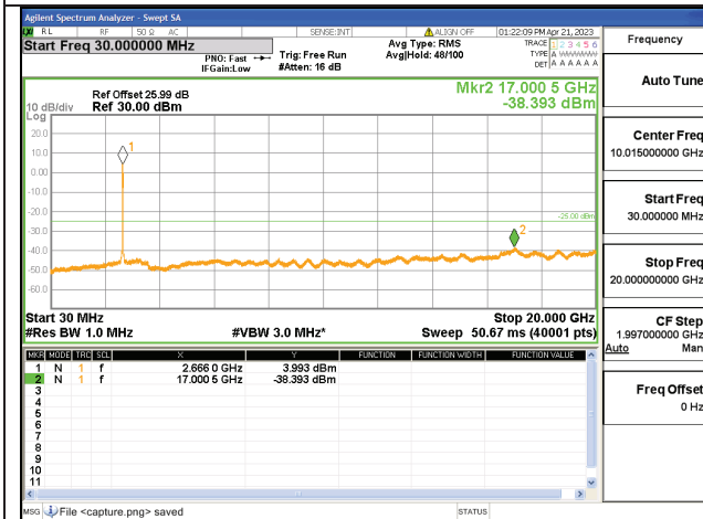
41C-30M-20G / 20+15MHz / QPSK / High CH / 100#0-75#0
