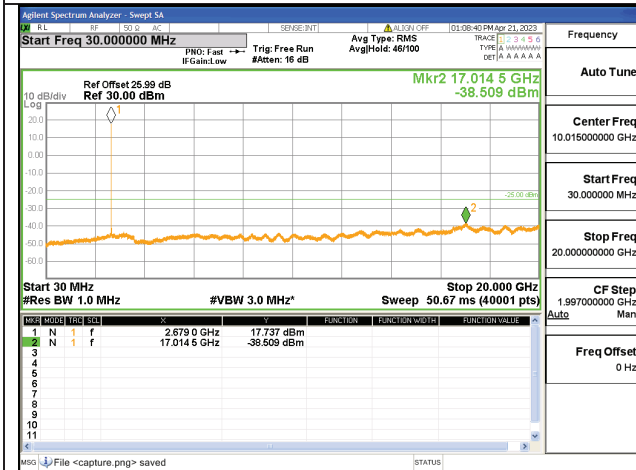
41C-30M-20G / 15+10MHz / QPSK / High CH / 1#74-1#0
