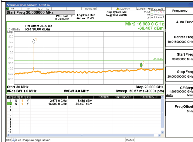
41C-30M-20G / 20+5MHz / QPSK / High CH / 100#0-25#0
