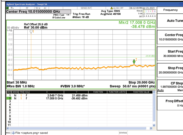
7C-30M-20G / 10+20MHz / QPSK / High CH / 1#49-1#0
