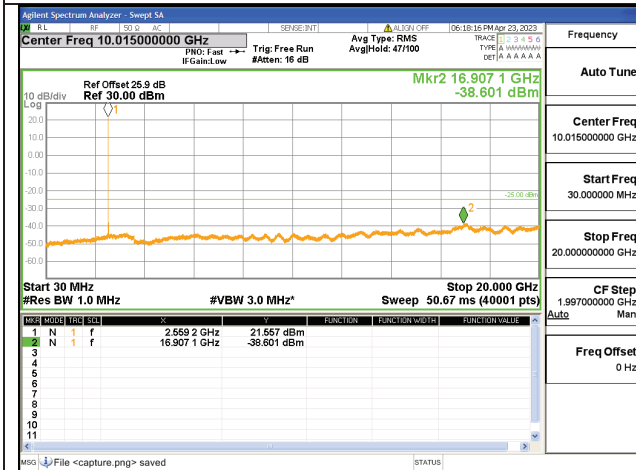
7C-30M-20G / 15+10MHz / QPSK / High CH / 1#74-1#0
