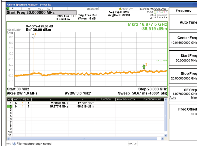
41C-30M-20G / 15+10MHz / QPSK / Low CH / 1#74-1#0
