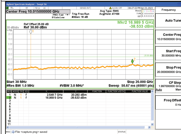
7C-30M-20G / 20+20MHz / QPSK / High CH / 1#99-1#0
