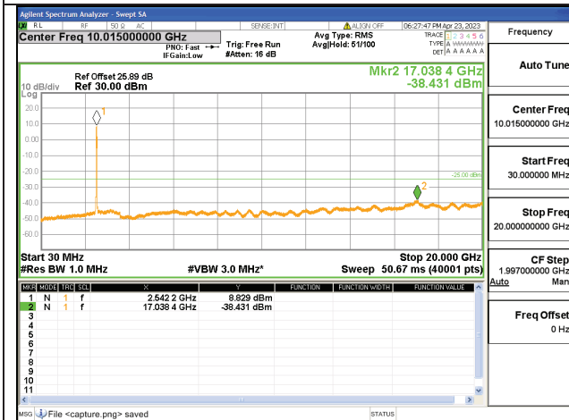
7C-30M-20G / 20+20MHz / QPSK / High CH / 100#0-100#0
