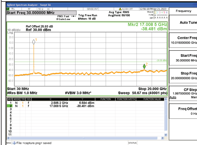
41C-30M-20G / 15+15MHz / QPSK / Mid CH / 75#0-75#0
