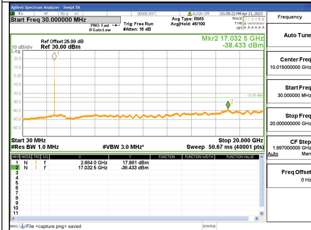
41C-30M-20G / 20+5MHz / QPSK / High CH / 1#99-1#0
