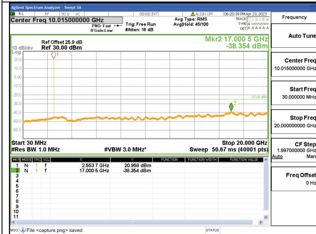
7C-30M-20G / 15+15MHz / QPSK / High CH / 1#74-1#0
