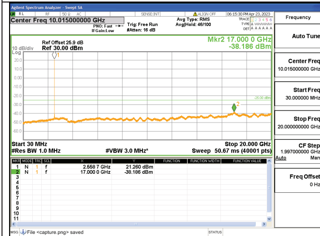
7C-30M-20G / 20+10MHz / QPSK / High CH / 1#99-1#0
