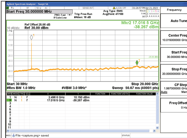
41C-30M-20G / 5+20MHz / QPSK / Low CH / #0-1#99
