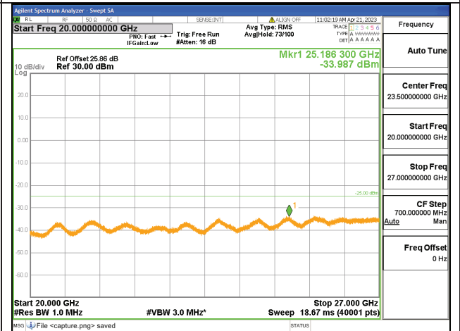
41C-20G-27G / 5+20MHz / QPSK / Low CH / #24-1#0
