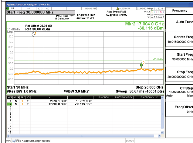
41C-30M-20G / 20+15MHz / QPSK / Mid CH / 1#99-1#0
