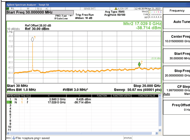
41C-30M-20G / 10+20MHz / QPSK / Mid CH / 50#0-100#0
