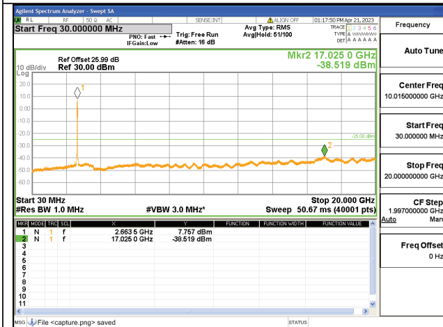
41C-30M-20G / 15+15MHz / QPSK / High CH / 75#0-75#0
