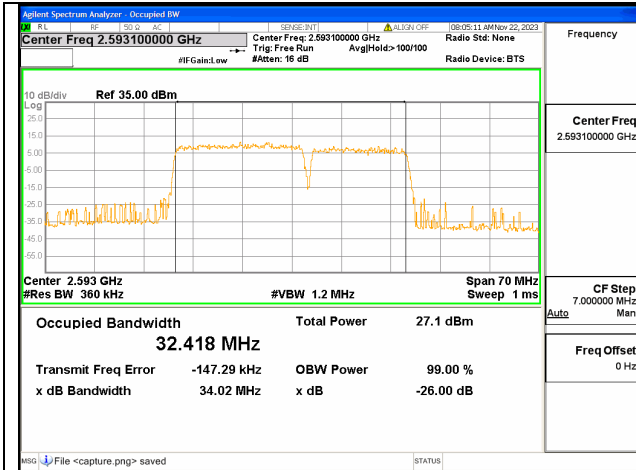
41C / 20+15MHz / 64QAM/ Mid CH
