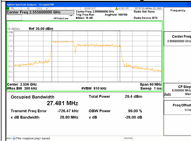
7C / 10+20MHz / 64QAM/ High CH
