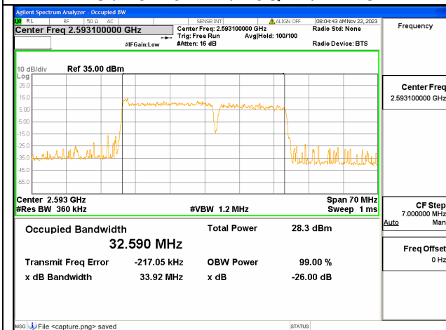
41C / 20+15MHz / QPSK/ Mid CH
