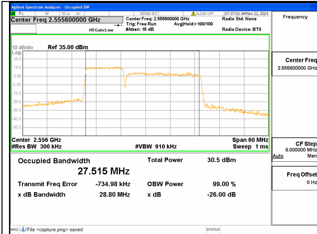
7C / 10+20MHz / QPSK/ High CH
