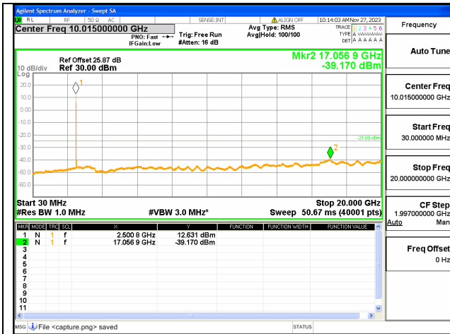
7C-30M-20G / 10+20MHz / QPSK / Low CH / 1@0-1@99
