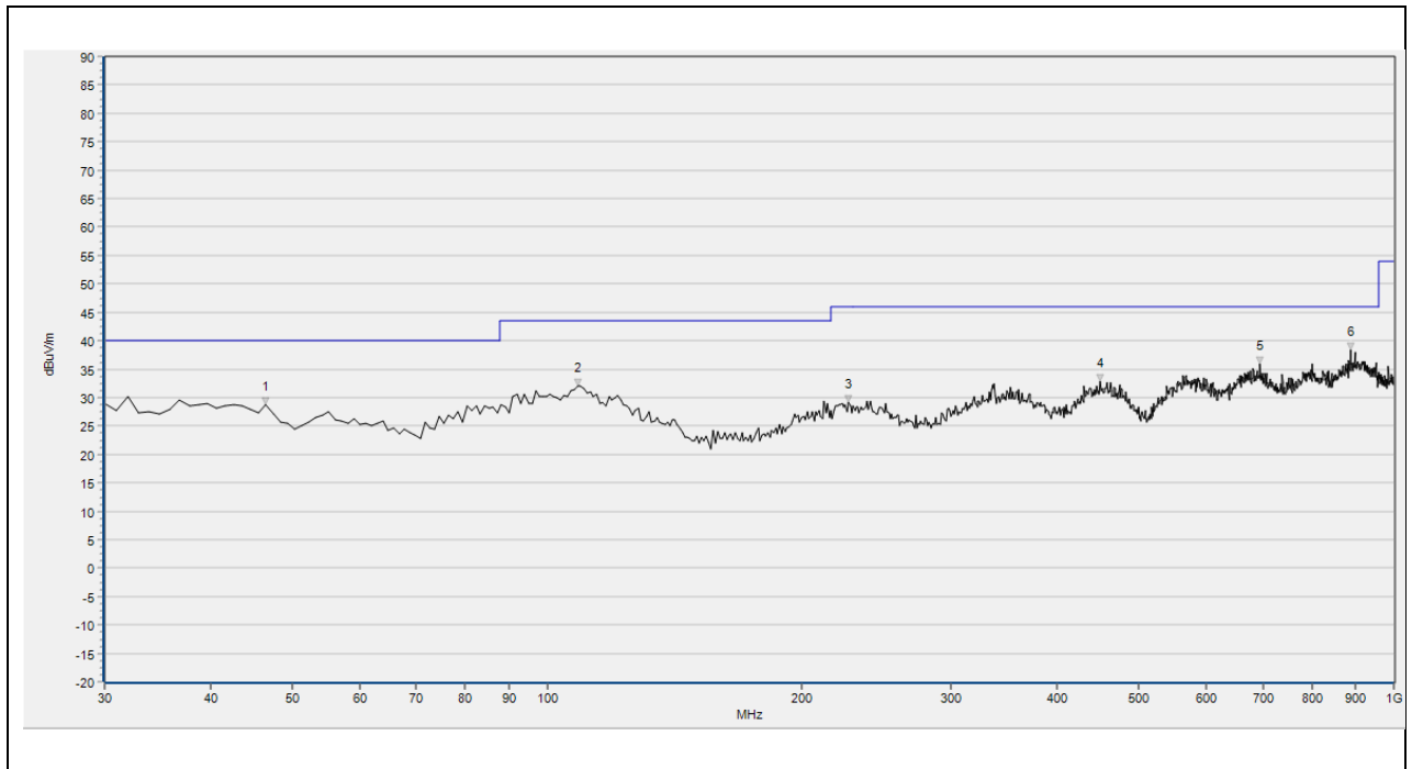
(30MHz – 1GHz, Test Antenna Vertical)
