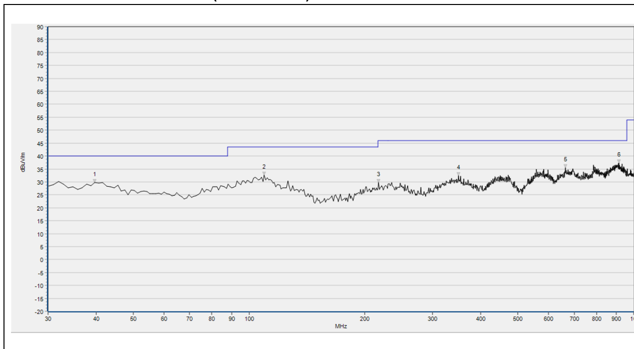
(30MHz – 1GHz, Test Antenna Horizontal)
