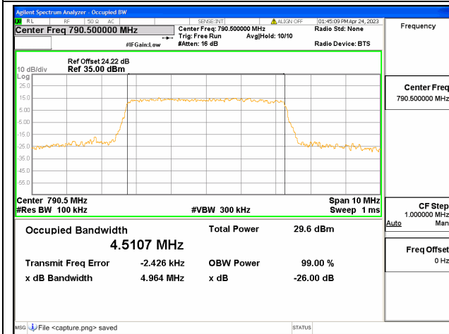
Band14 / 5MHz / 64QAM/ Low CH
