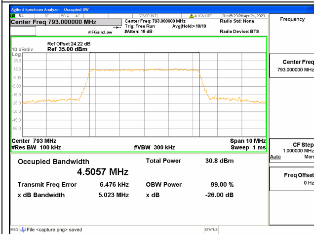
Band14 / 5MHz / 16QAM/ Mid CH
