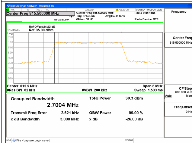
Band26 Part90 / 3MHz / 16QAM/ Low CH
