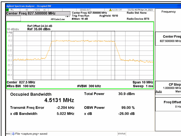
Band18 part22 / 5MHz / QPSK/ High CH
