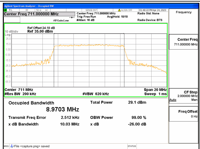
Band17 / 10MHz / 64QAM/ High CH
