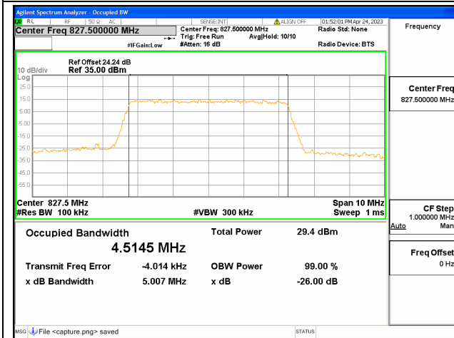
Band18 part22 / 5MHz / 64QAM/ High CH
