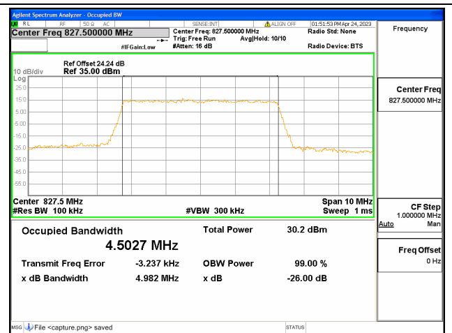
Band18 part22 / 5MHz / 16QAM/ High CH
