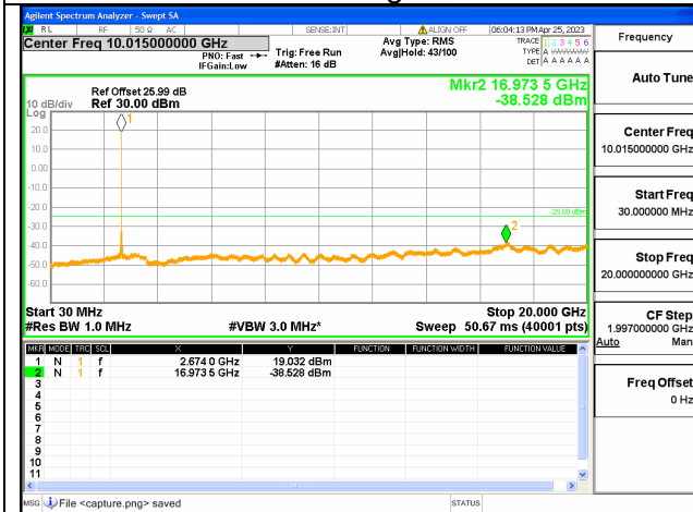
Band41C-30M-20G / 15+15MHz /1RB+1RB/ QPSK / High CH
