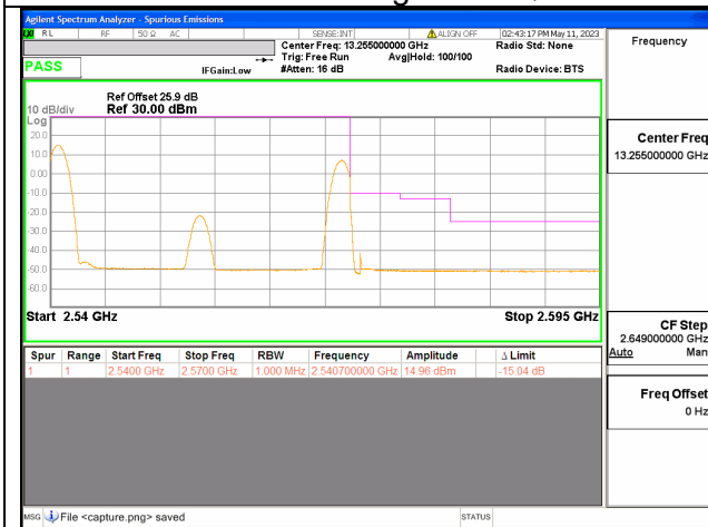
Band7C / 15+15MHz / High CH / QPSK / 1 RB
