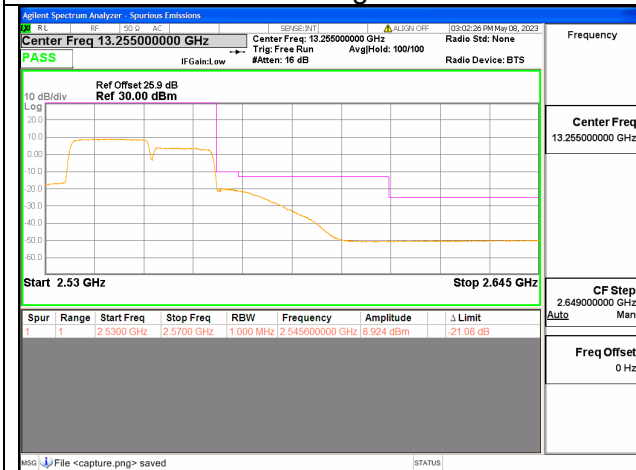
Band7C / 20+15MHz / High CH / QPSK / 100 RB
