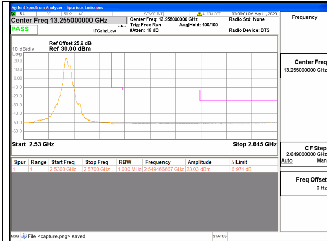
Band7C / 15+20MHz / High CH / QPSK / 1 RB
