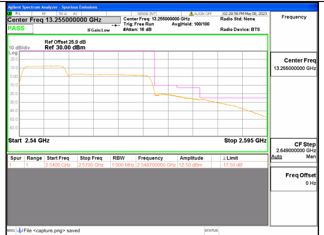
Band7C / 10+20MHz / High CH / QPSK / 50 RB
