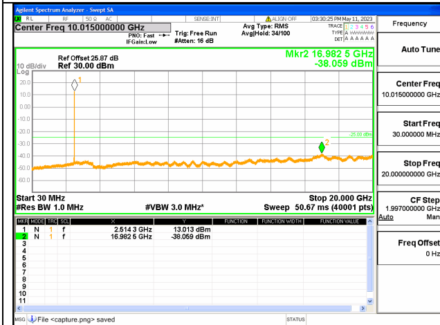
Band7C-30M-20G / 15+15MHz / 1RB+1RB / QPSK / Low CH
