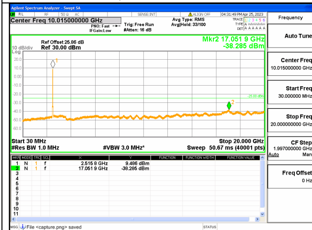
Band41C-30M-20G / 20+5MHz / 100RB+25RB / QPSK / Low CH
