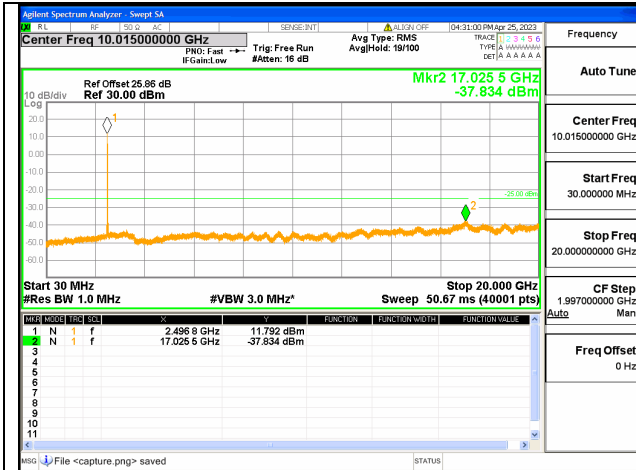
Band41C-30M-20G / 20+5MHz / 1RB+1RB / QPSK / Low CH
