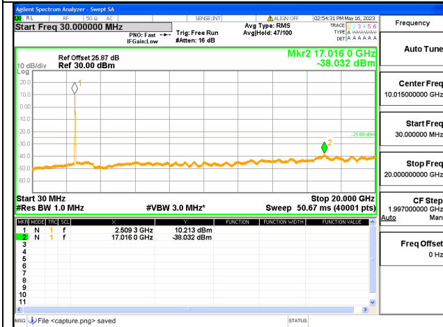
Band7C-30M-20G / 20+20MHz / 100RB+100RB/ QPSK / Low CH
