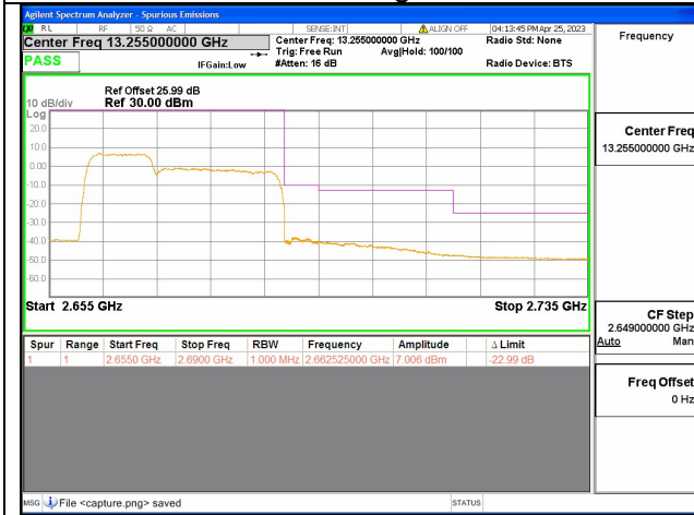
Band41C / 10+20MHz / High CH / QPSK / 50 RB
