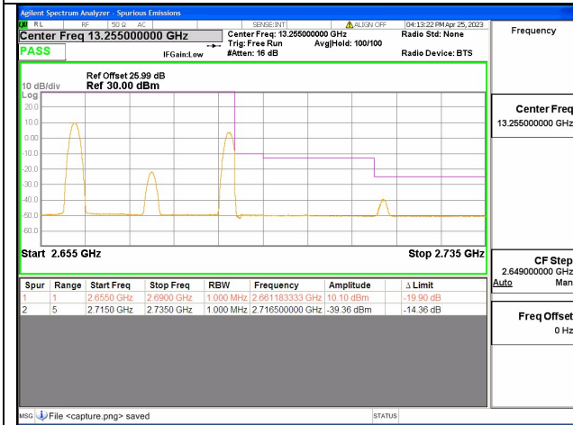
Band41C / 10+20MHz / High CH / QPSK / 1 RB
