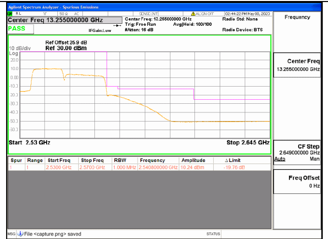
Band7C / 15+20MHz / High CH / QPSK / 75 RB
