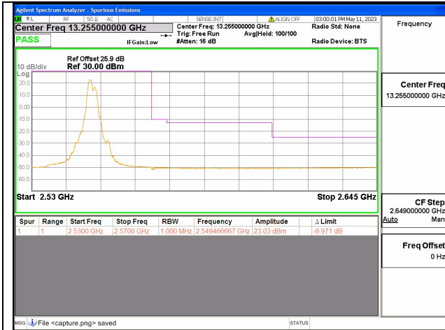
Band7C / 15+20MHz / High CH / QPSK / 1 RB
