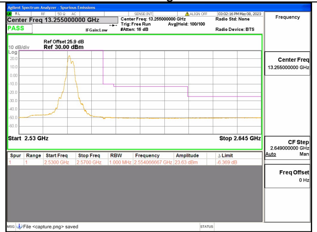
Band7C / 20+15MHz / High CH / QPSK / 1 RB
