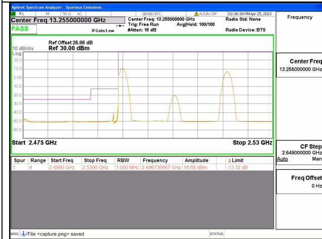
Band41C / 10+15MHz / Low CH / QPSK / 1 RB
