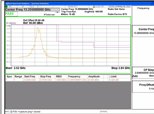
Band7C / 20+20MHz / High CH / QPSK / 1 RB
