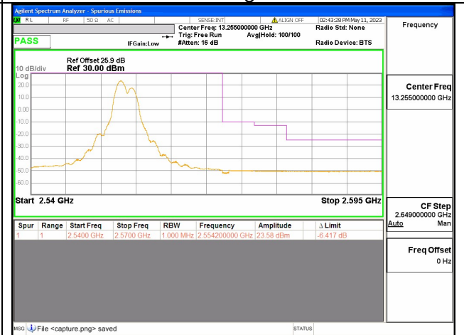
Band7C / 15+15MHz / High CH / QPSK / 75 RB
