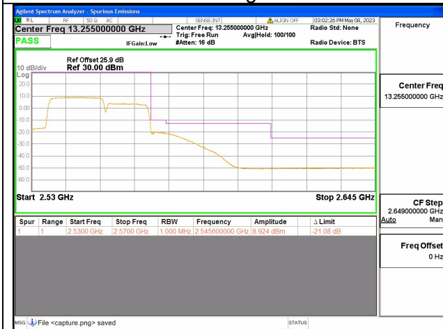
Band7C / 20+15MHz / High CH / QPSK / 100 RB
