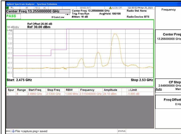
Band41C / 20+5MHz / Low CH / QPSK / 1 RB
