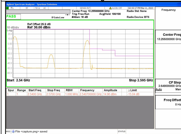
Band7C / 15+15MHz / High CH / QPSK / 1 RB
