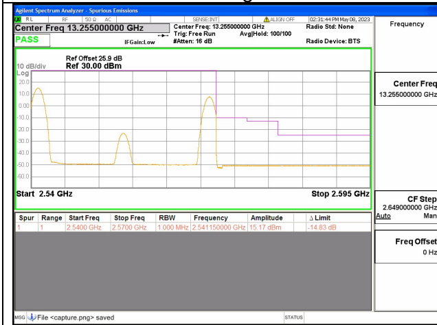
Band7C / 10+20MHz / High CH / QPSK / 1 RB
