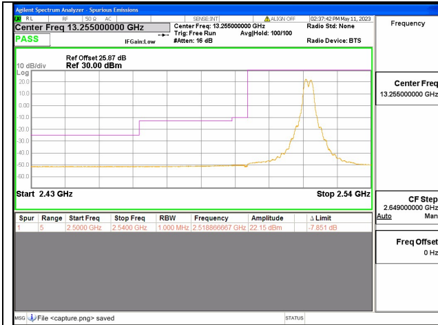
Band7C / 20+15MHz / Low CH / QPSK / 1 RB
