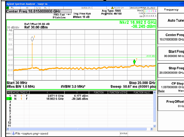
Band41C-30M-20G / 20+10MHz / 100RB+50RB / QPSK / High CH
