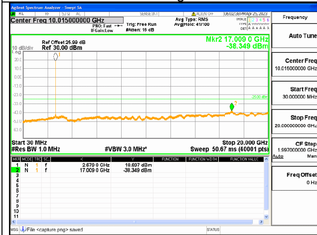
Band41C-30M-20G / 20+10MHz / 1RB+1RB / QPSK / High CH
