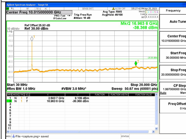
Band41C-30M-20G / 10+20MHz / 50RB+100RB / QPSK / Mid CH
