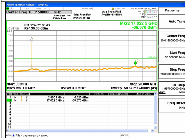
Band41C-30M-20G / 20+10MHz / 100RB+50RB / QPSK / Mid CH
