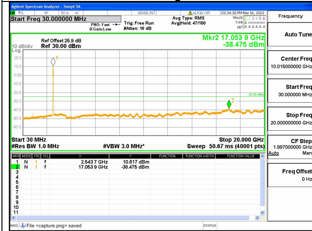
Band7C-30M-20G / 20+15MHz /100RB+75RB/ QPSK / High CH
