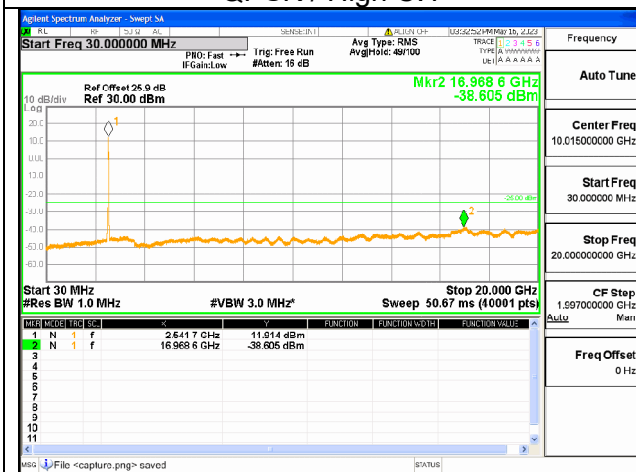
Band7C-30M-20G / 15+20MHz / 75RB+100RB / QPSK / High CH
