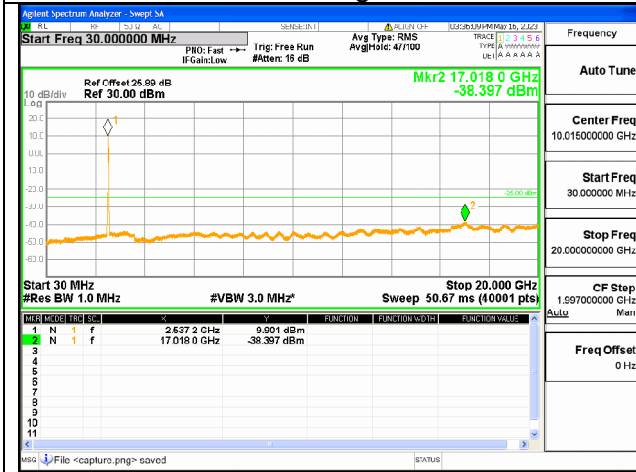
Band7C-30M-20G / 20+20MHz / 100RB+100RB / QPSK / High CH
