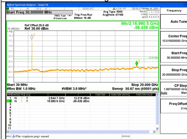
Band7C-30M-20G / 15+15MHz / 75RB+75RB / QPSK / High CH
