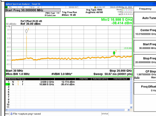
Band7C-30M-20G / 15+20MHz / 75RB+100RB / QPSK / Mid CH
