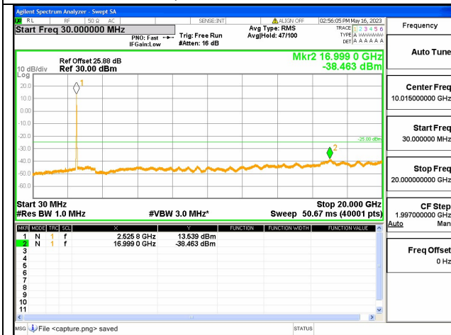
Band7C-30M-20G / 10+20MHz /50RB+100RB/ QPSK / Mid CH
