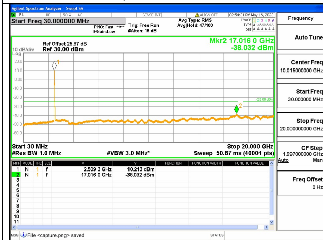
Band7C-30M-20G / 20+20MHz / 100RB+100RB / QPSK / Low CH
