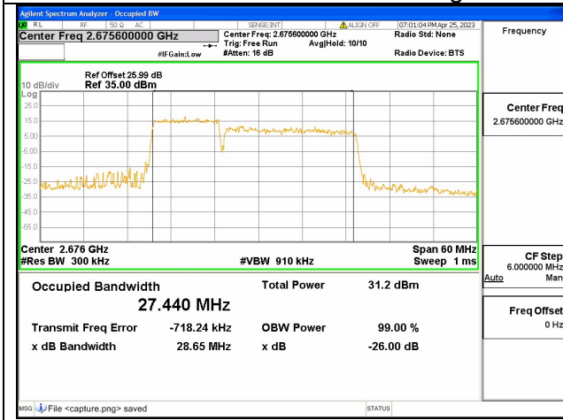
Band41C / 10+20MHz / 64QAM/ High CH
