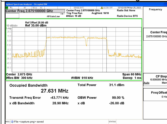
Band41C / 20+10MHz / 16QAM/ High CH
