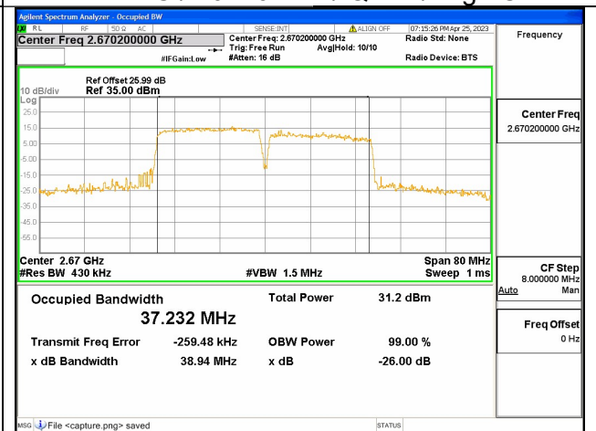
Band41C / 20+20MHz / 16QAM/ High CH
