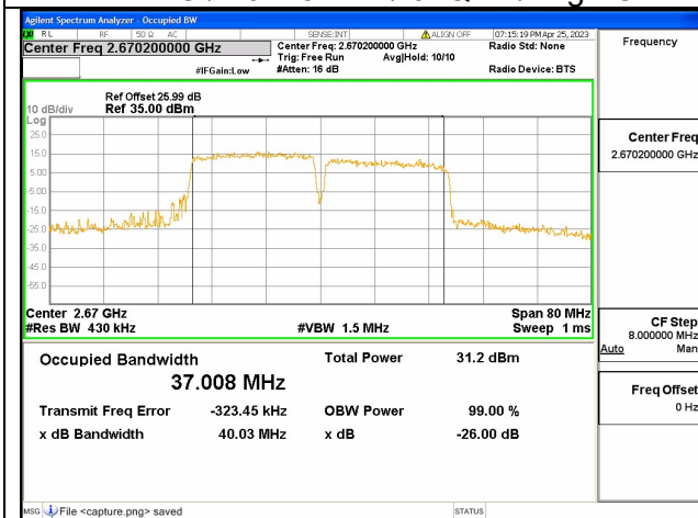
Band41C / 20+20MHz / 64QAM/ High CH
