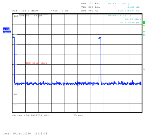
Figure 8.6-1: One transmission within 100 ms
