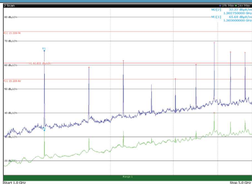
Antenna in vertical polarization – EUT in vertical position
