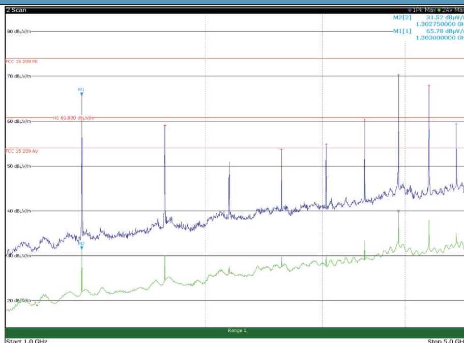
Antenna in vertical polarization – EUT in horizontal position
