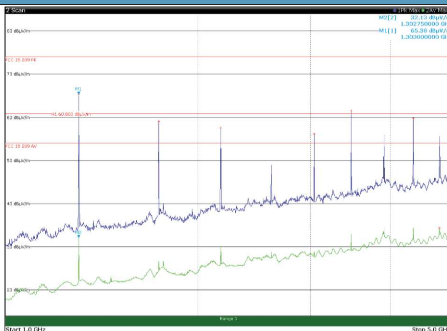
Antenna in horizontal polarization – EUT in vertical position
