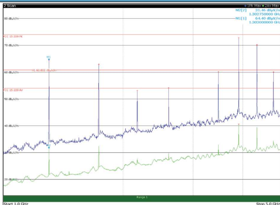
Antenna in horizontal polarization – EUT in horizontal position
