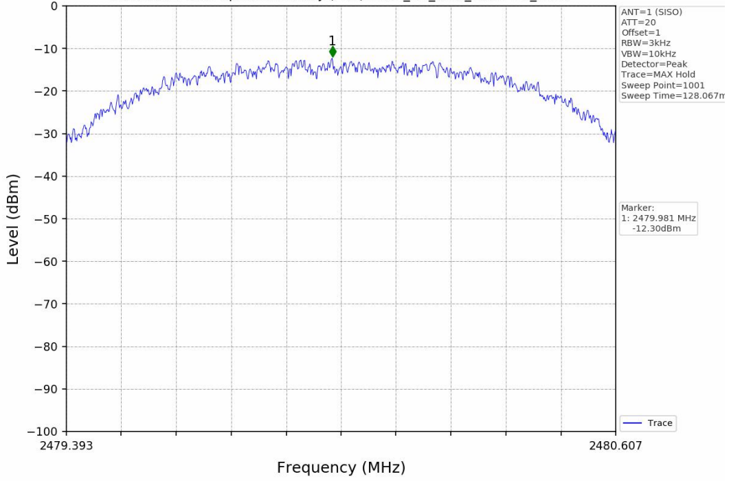
Maximum Power Spectral Density (PSD) NTVN_2M_SISO_2480MHz_ANT1
