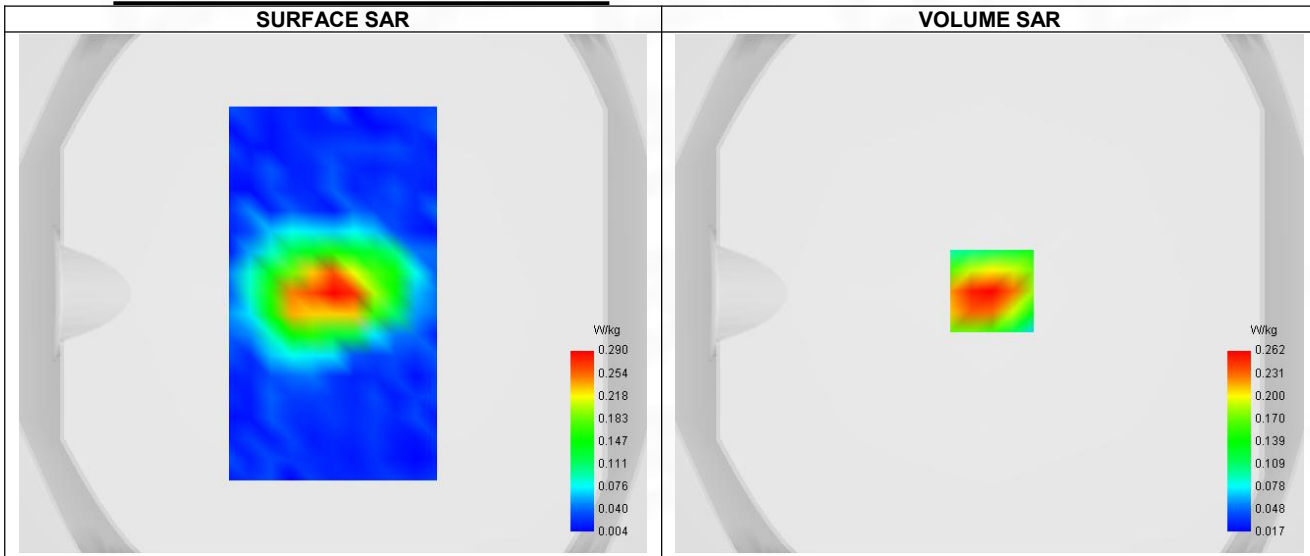
Maximum location: X=1.00, Y=1.00 ; SAR Peak: 0.36 W/kg
