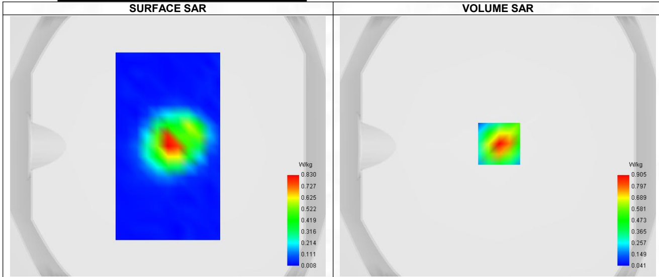
Maximum location: X=1.00, Y=2.00 ; SAR Peak: 1.45 W/kg
