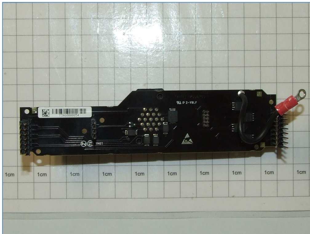
Board mod. 810 Connectors – Top
