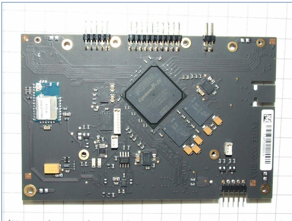
Board mod. 811 Carrier - Bottom
