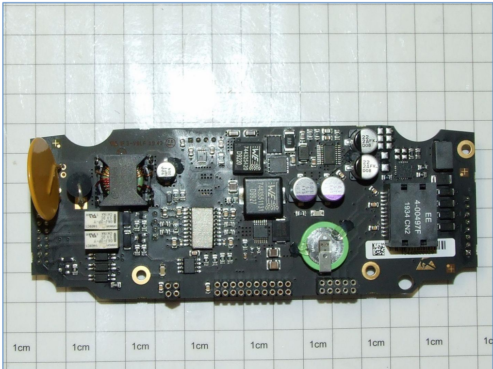
Board mod. 809 Power – Top
