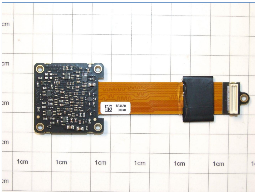
Board mod. 795 Image Sensor Color – Bottom
