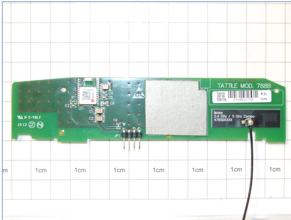
Board mod. 788 GPS – Top
