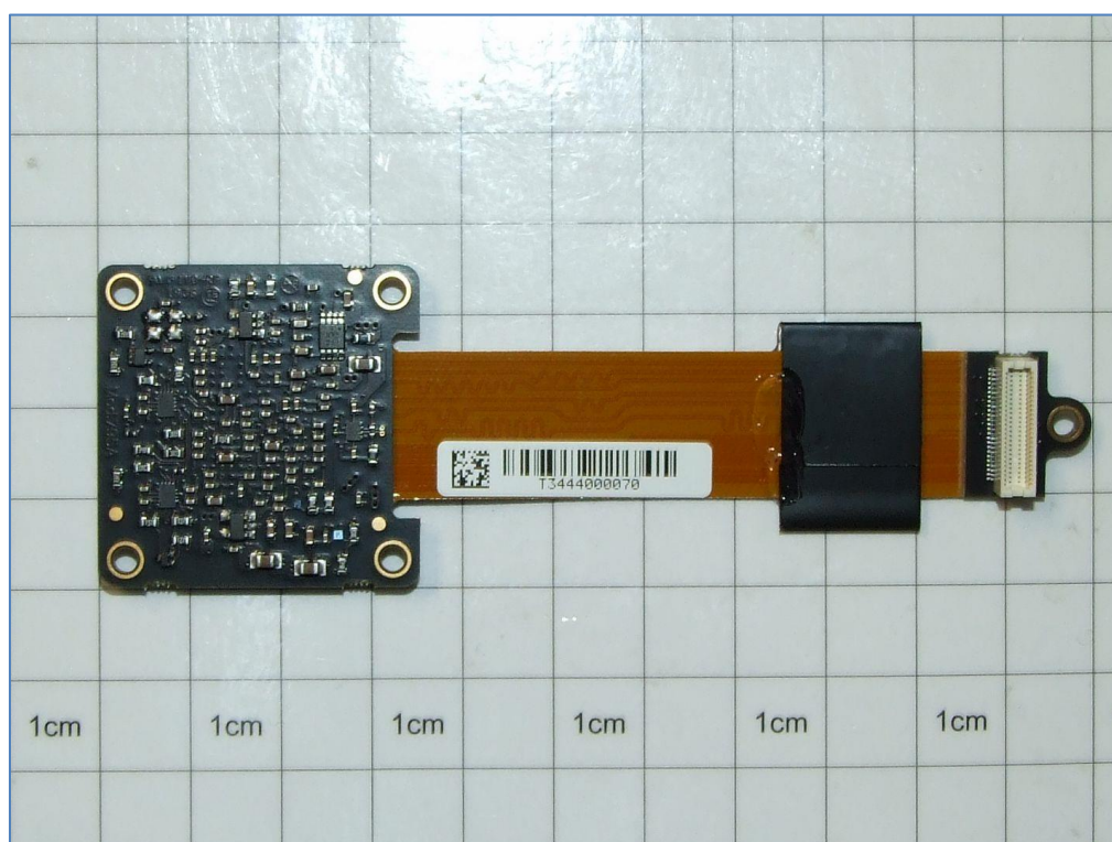
Board mod. 795 Image Sensor Mono – Bottom
