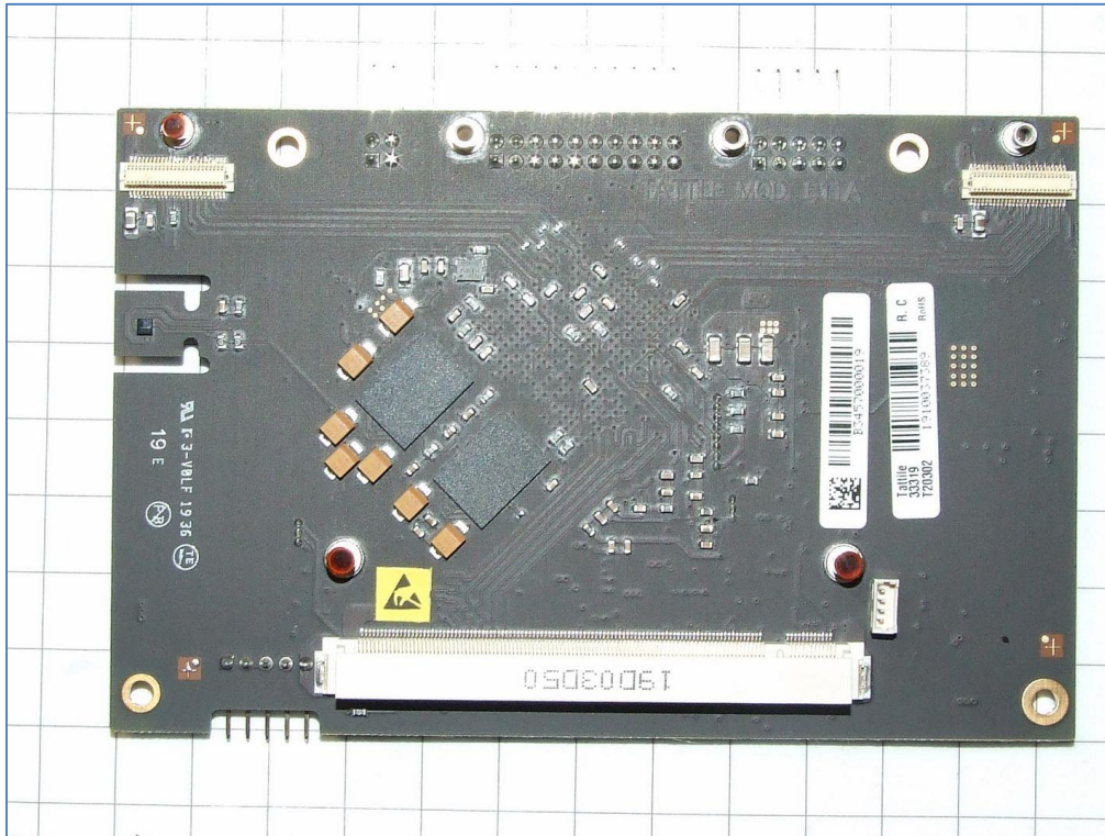
Board mod. 811 Carrier - Top
