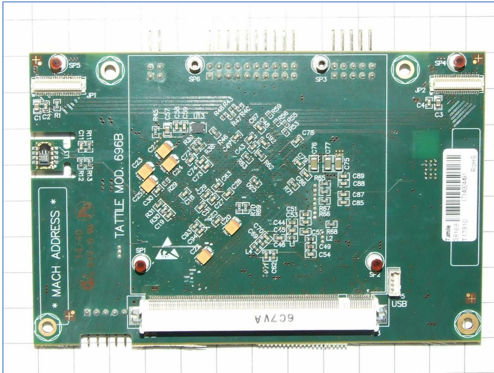
Board mod. 696 Carrier - Top
