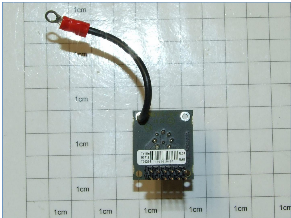
Board mod. 812 Connectors – Top
