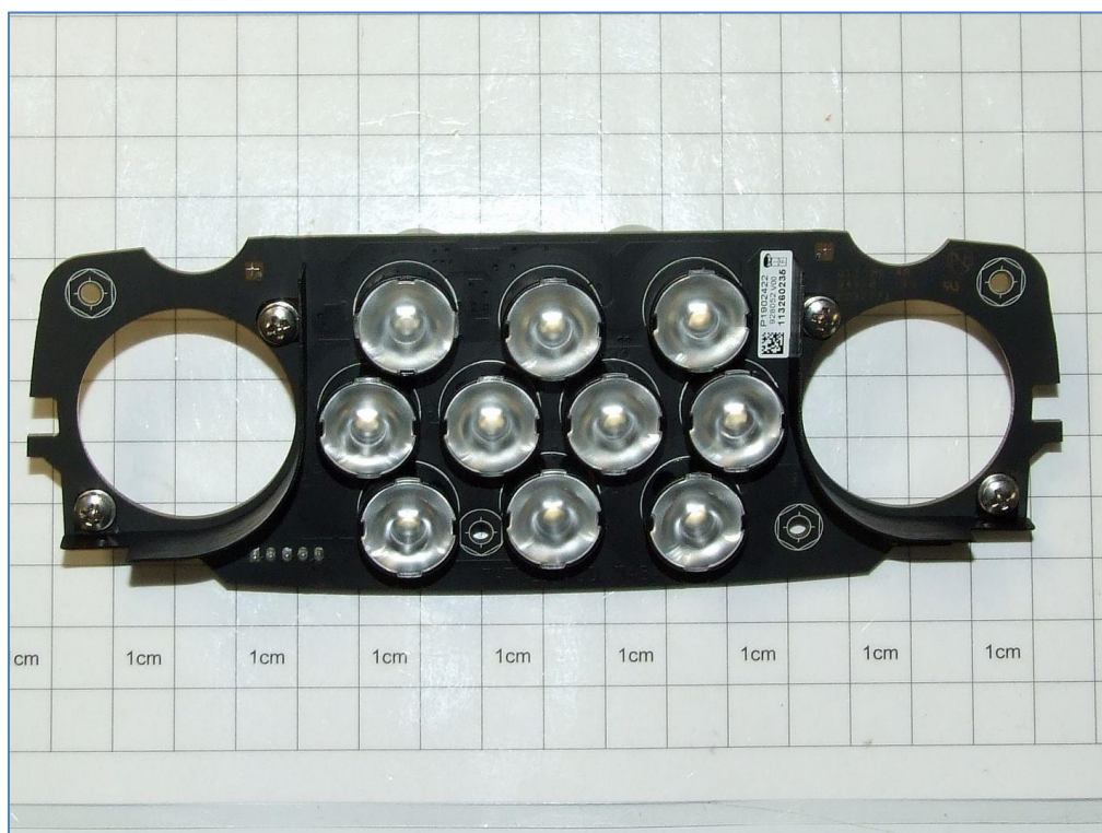
Board mod. 748 Illuminator – Bottom
