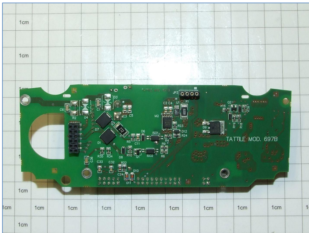
Board mod. 697 Power – Bottom
