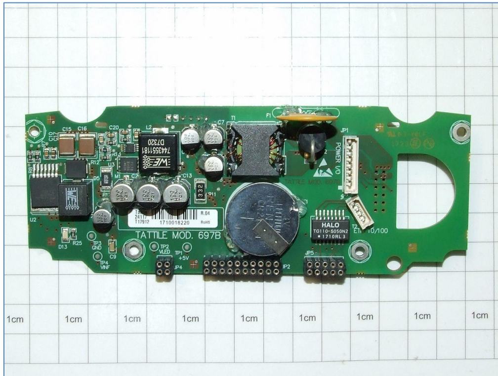
Board mod. 697 Power – Top
