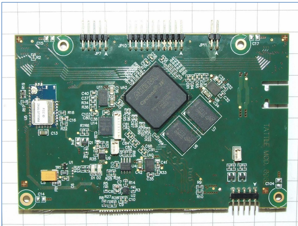
Board mod. 696 Carrier - Bottom
