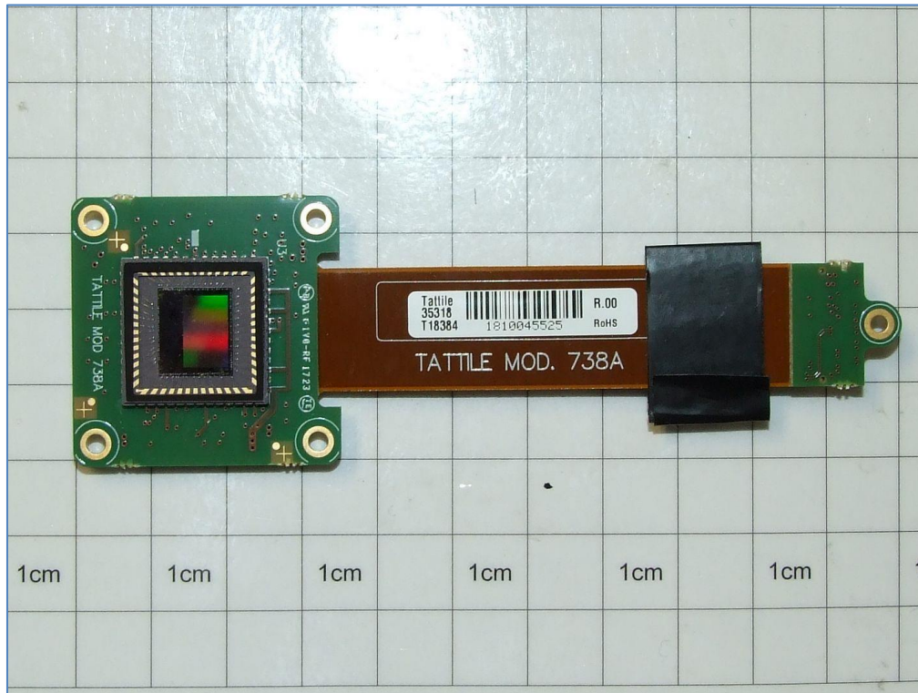
Board mod. 738 Image Sensor Color – Top
