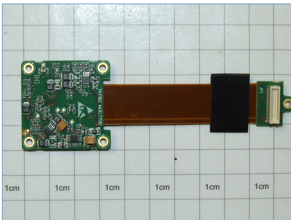
Board mod. 770 Image Sensor Mono – Bottom
