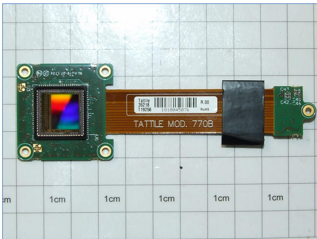
Board mod. 770 Image Sensor Mono – Top
