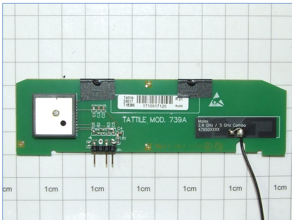
Board mod. 739 GPS – Top
