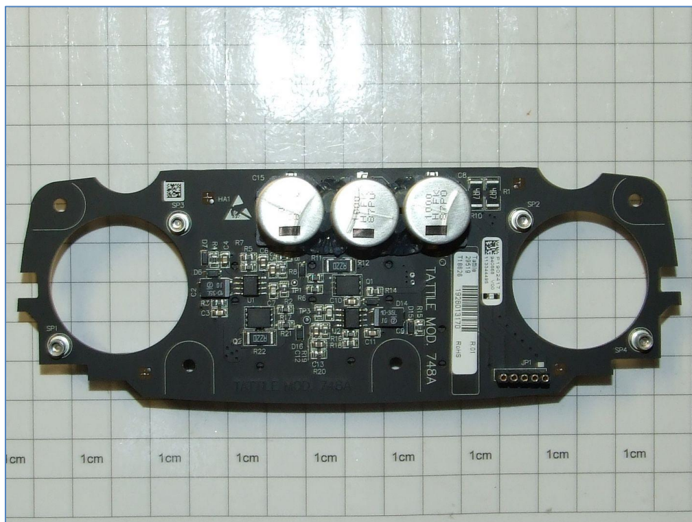
Board mod. 748 Illuminator – Top
