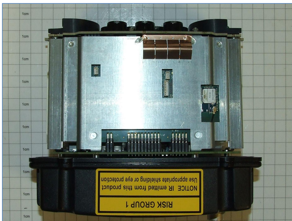
Bottom (with rear cover)
