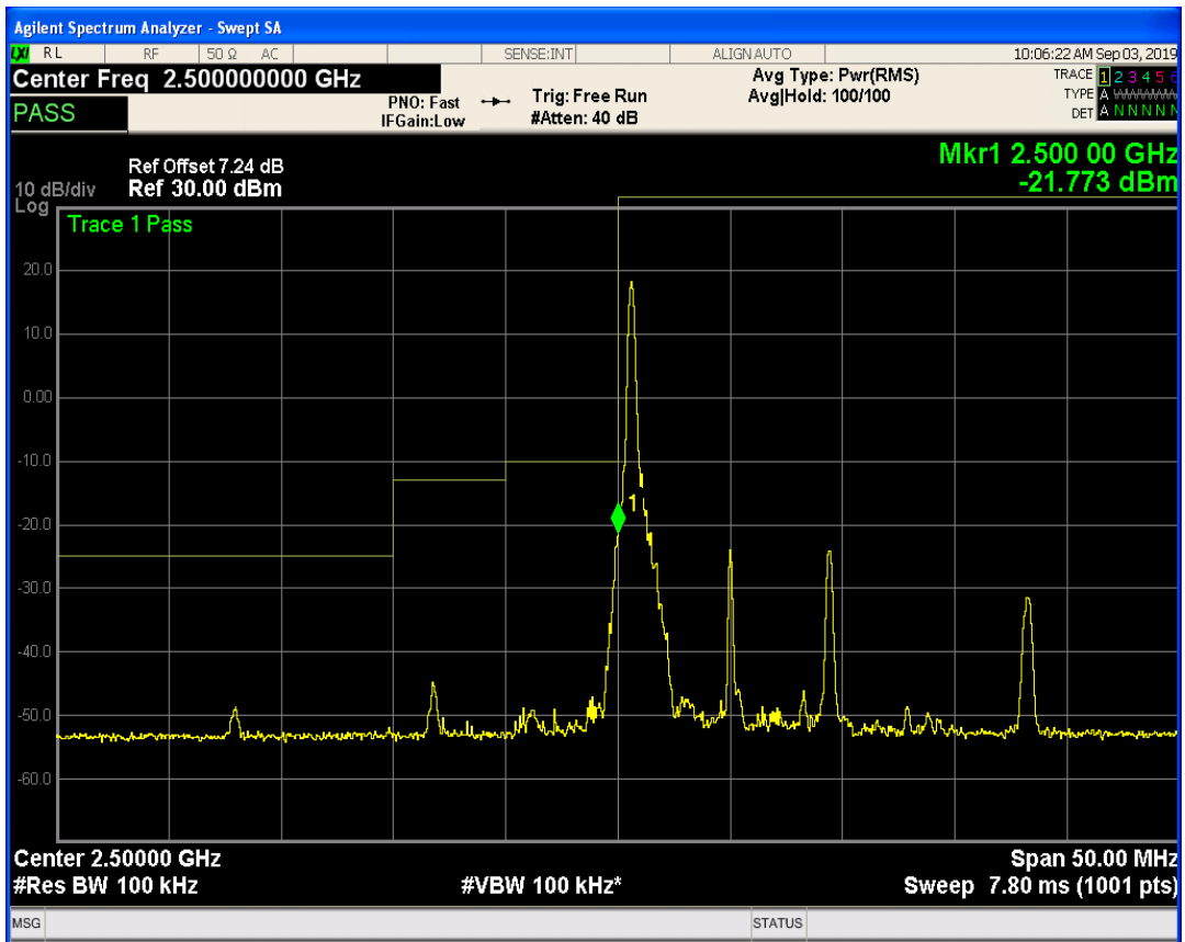
LTE Band7 QAM16 BW=10MHz Channel=20800 RB Size=1 Position=#Max
