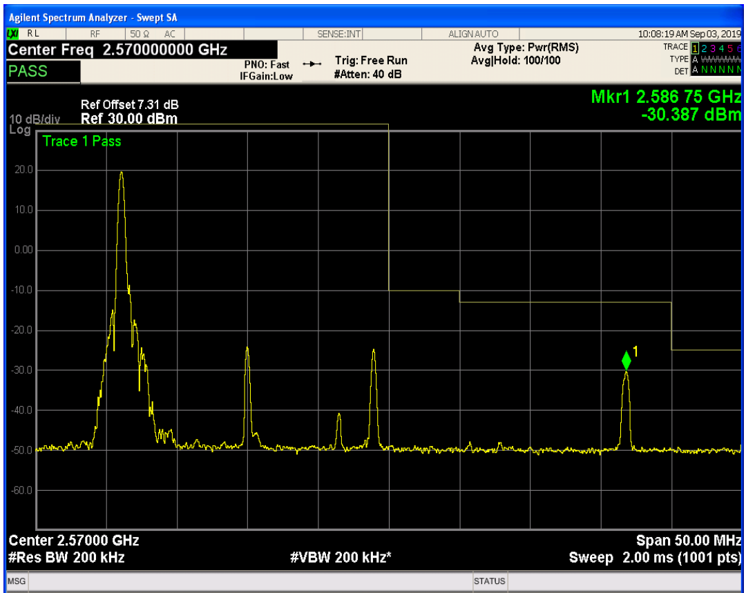
LTE Band7 QAM16 BW=20MHz Channel=21350 RB Size=1 Position=#Max
