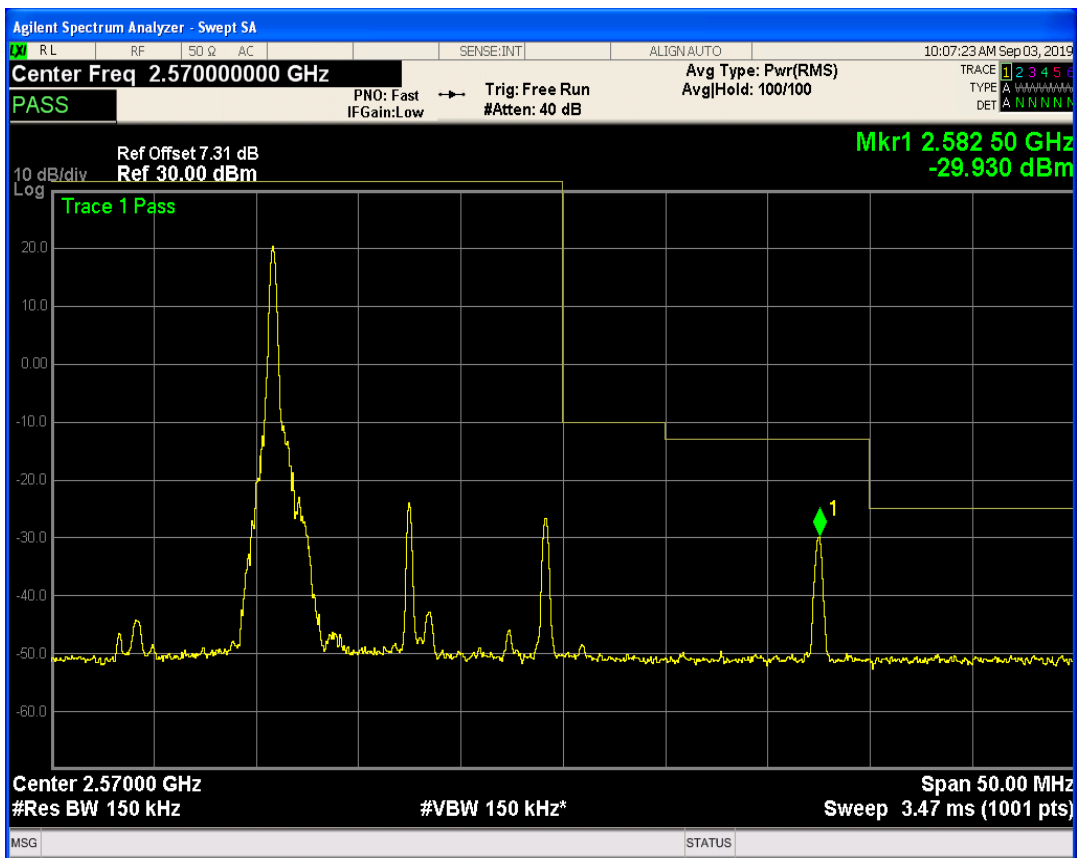
LTE Band7 QPSK BW=15MHz Channel=21375 RB Size=1 Position=#Max
