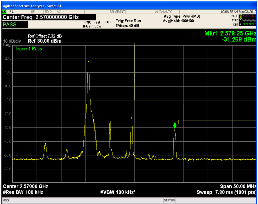
LTE Band7 QPSK BW=10MHz Channel=21400 RB Size=1 Position=#Max
