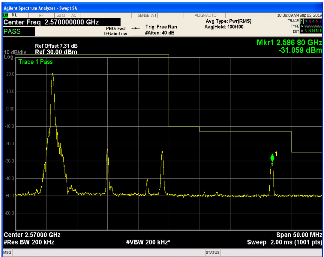
LTE Band7 QPSK BW=20MHz Channel=21350 RB Size=1 Position=#Max
