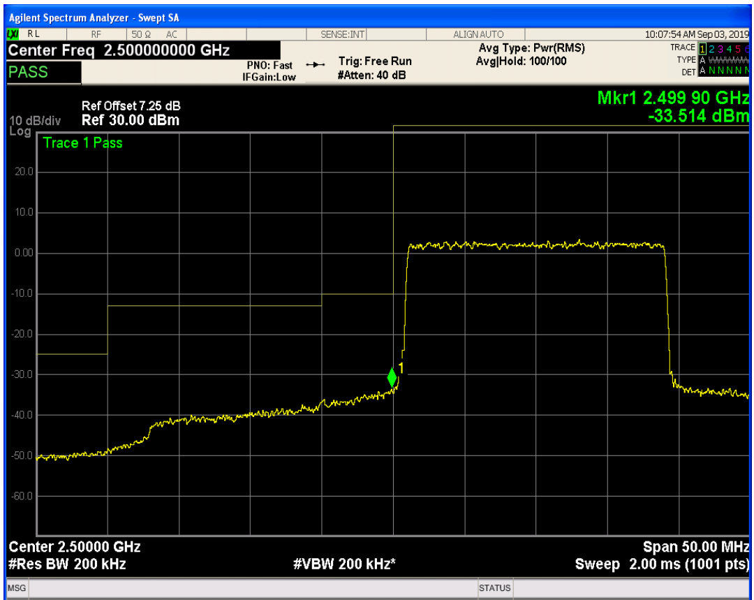
LTE Band7 QPSK BW=20MHz Channel=20850 RB Size=1 Position=#Max
