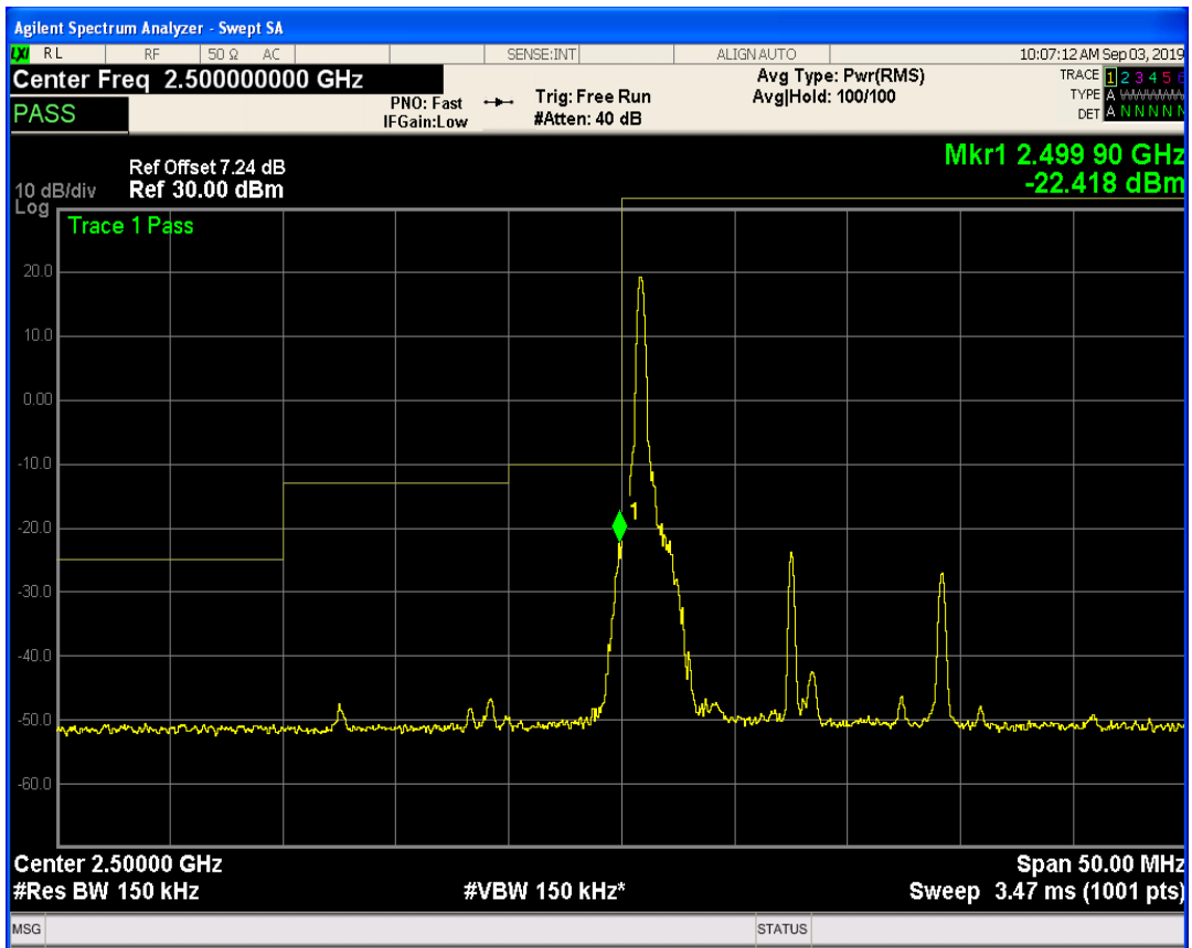
LTE Band7 QAM16 BW=15MHz Channel=20825 RB Size=1 Position=#Max
