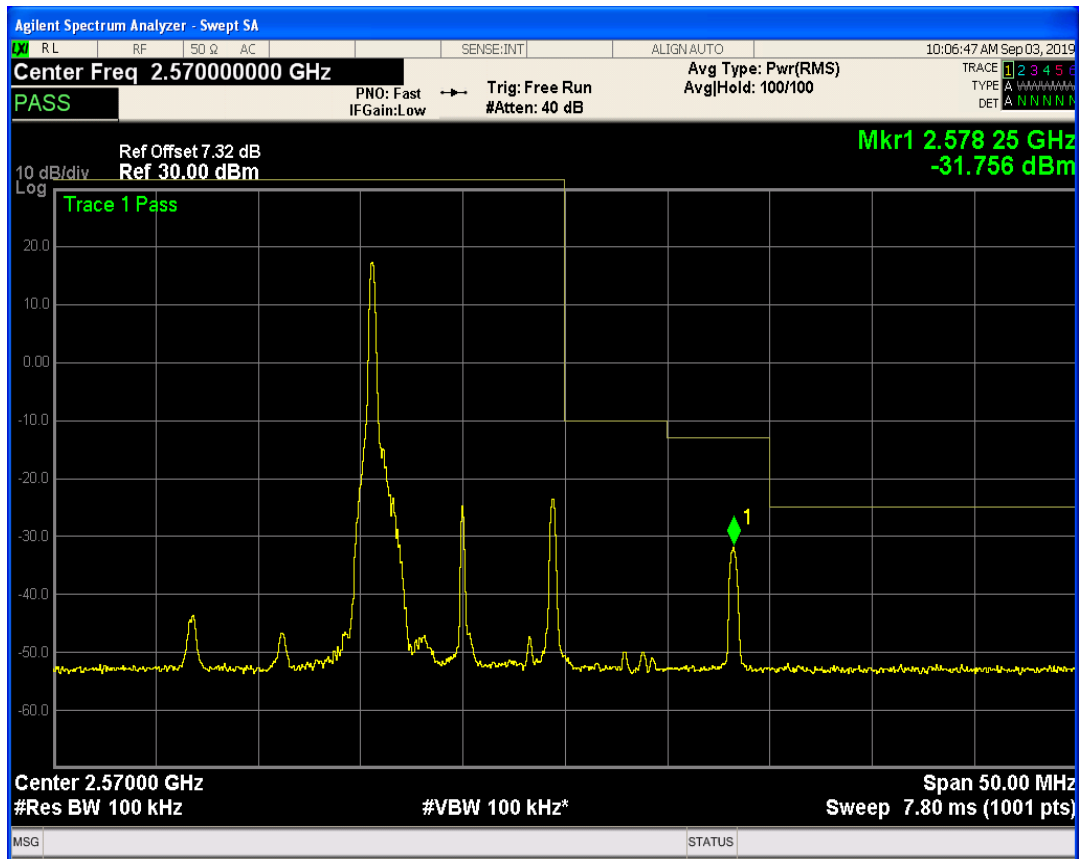
LTE Band7 QAM16 BW=10MHz Channel=21400 RB Size=1 Position=#Max
