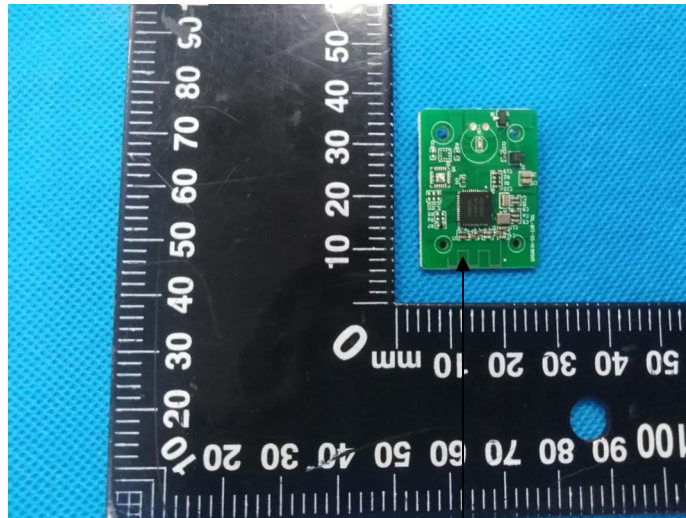
BT Antenna
