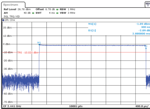
Channel 39 / 2441 MHz - DH3
