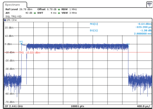
Channel 39 / 2441 MHz - 2DH3
