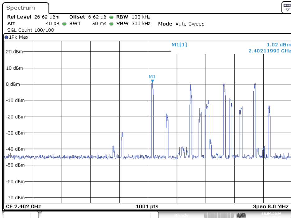
Band Edge NVNT 1-DH1 2402MHz Ant1 Hopping Ref
