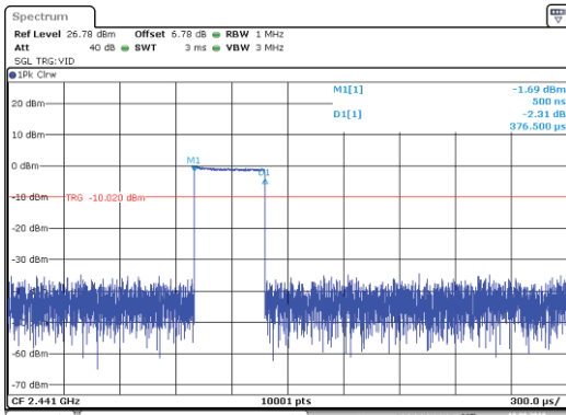
Channel 39 / 2441 MHz - DH1
