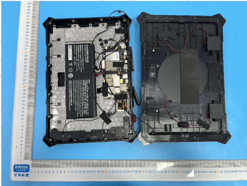
ANT 1 BT+WIFI+GNSS(RX)
