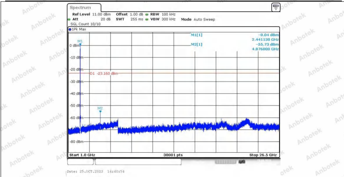
11AX20SISO_Ant2_2437_0~Reference
