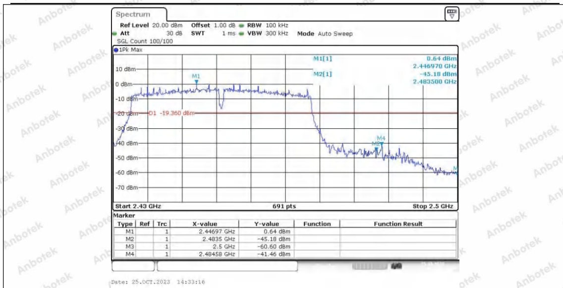
11N40SISO_Ant2_High_2452
