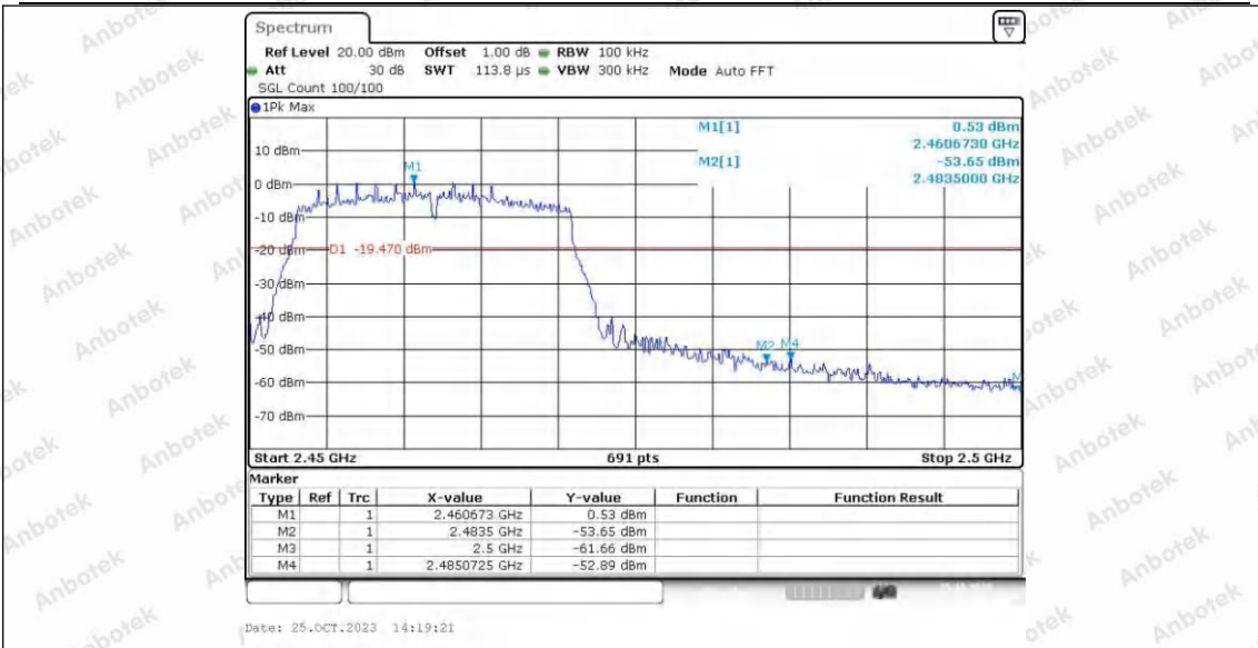
11N20SISO_Ant2_High_2462
