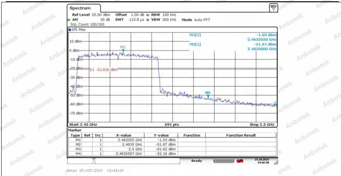
11AX20SISO_Ant2_High_2462
