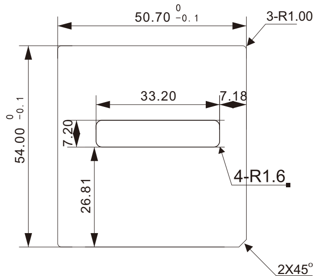
(Dimensional drawing)
