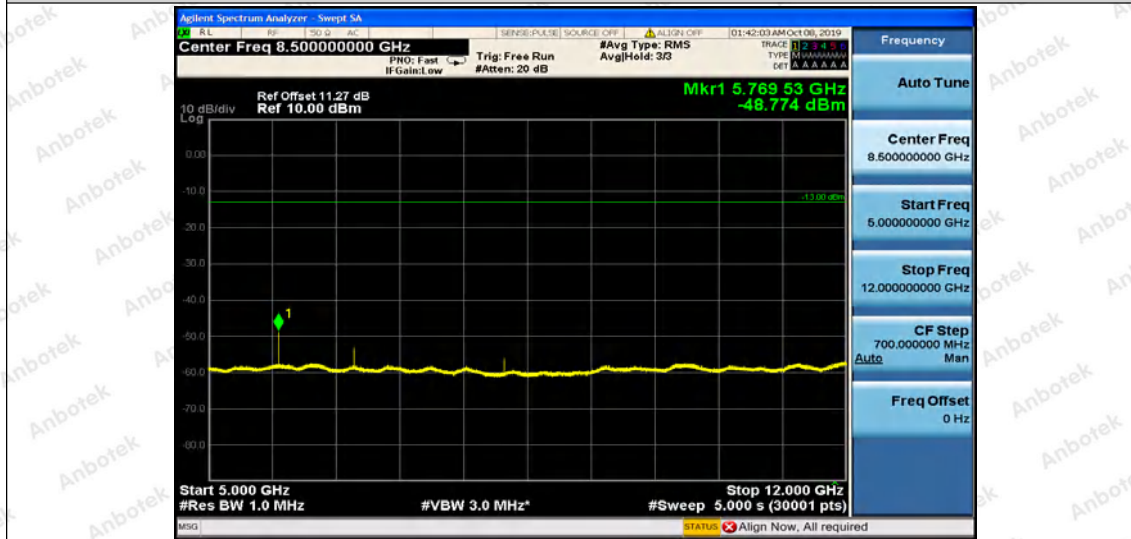
GPRS850-128-5000~12000
