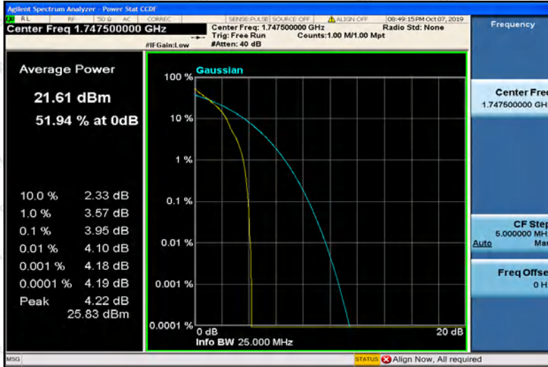
Band4-15MHz-QPSK-20325-175RB#0
