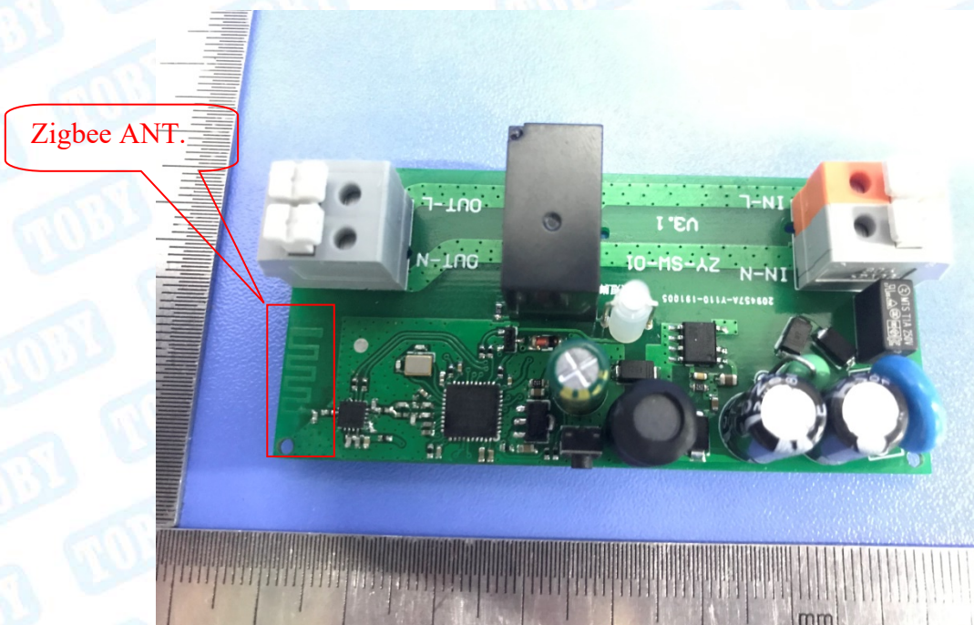
Photo 10 Appearance of PCB
