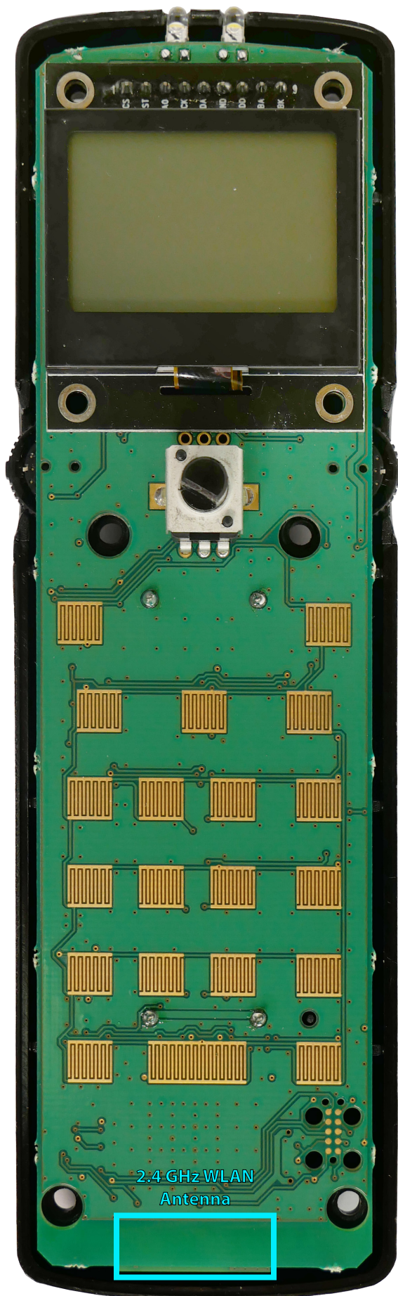
PCB Viewed from Front (Front of case removed)
