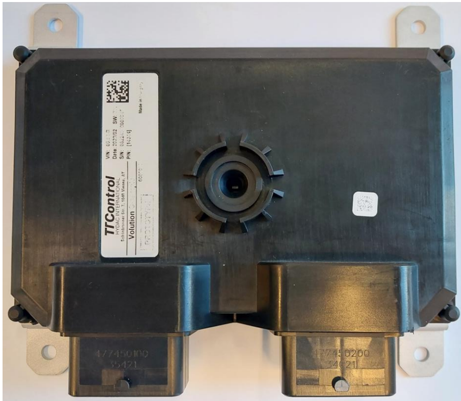
Figure 3: Top view
