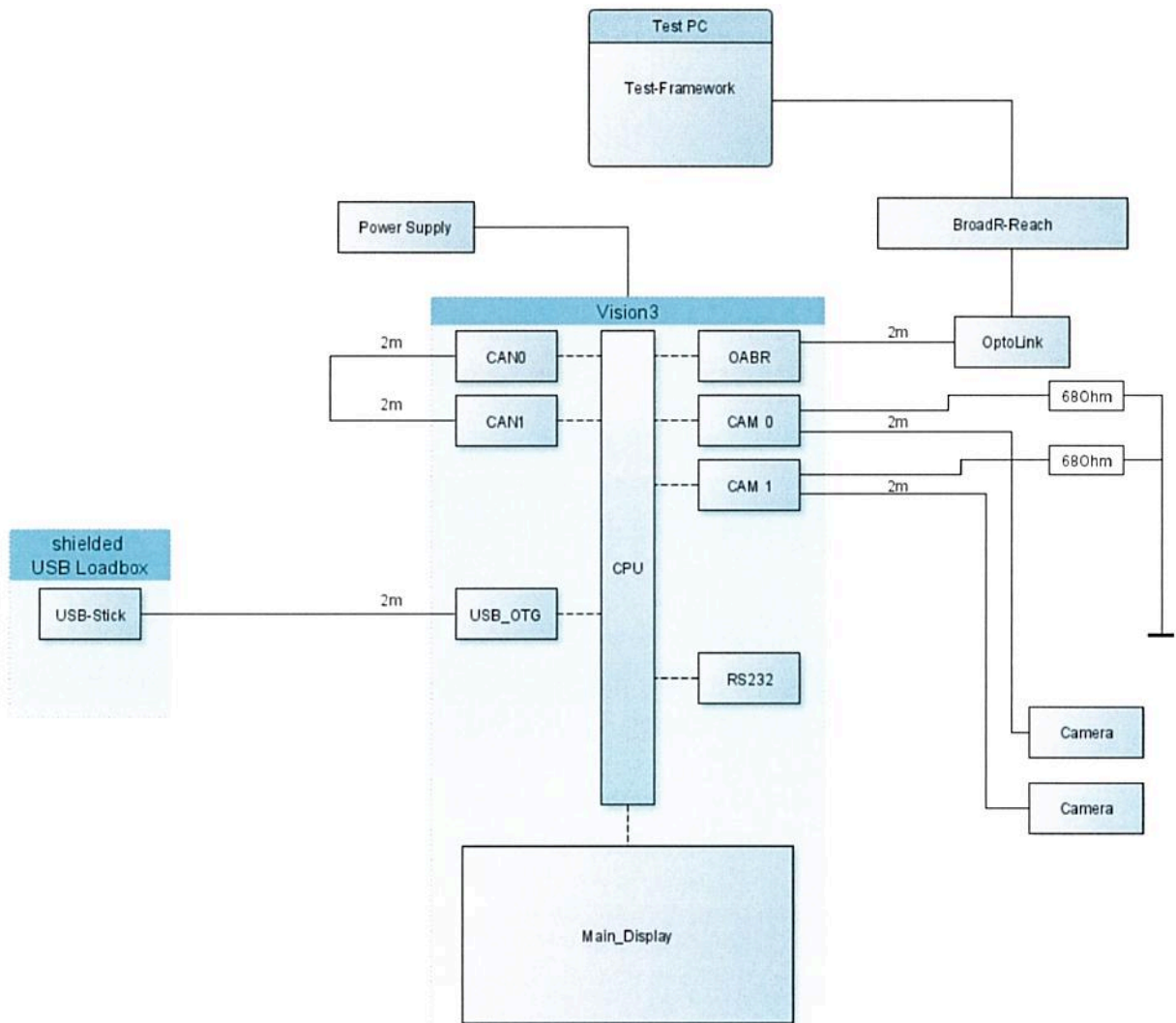
Figure 1: DUT test setup
