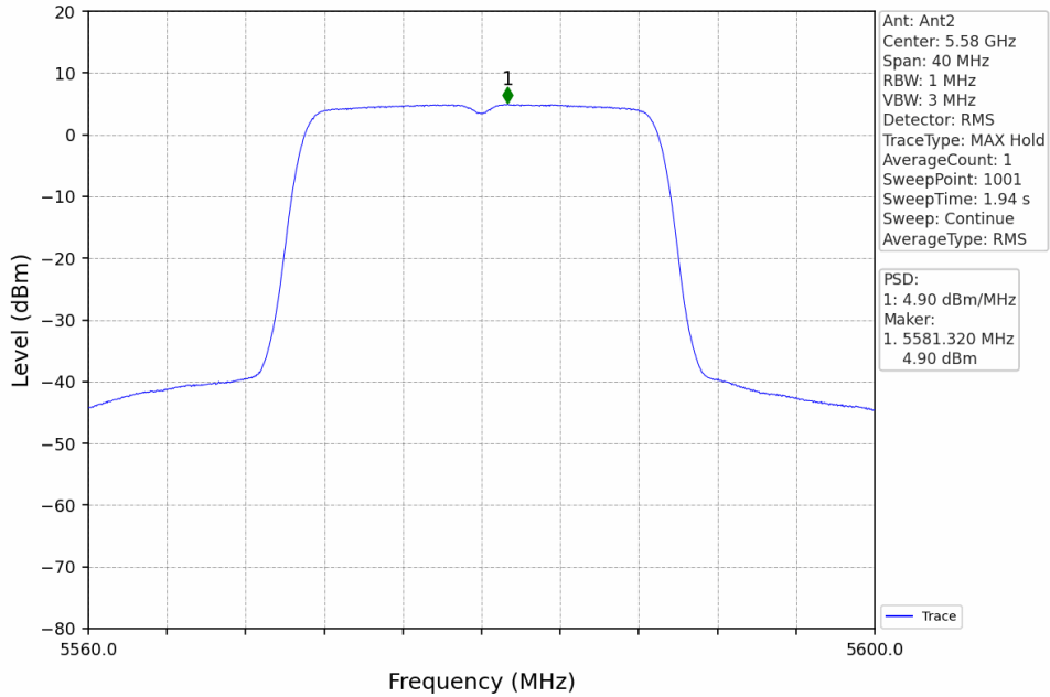
802.11ac(VHT20)_MCH_5580MHz_MIMO_NTNV
