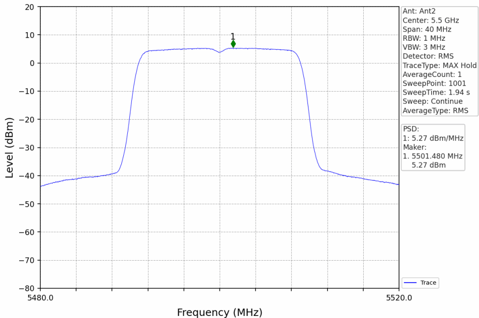
802.11ac(VHT20)_LCH_5500MHz_Ant2_NTNV
