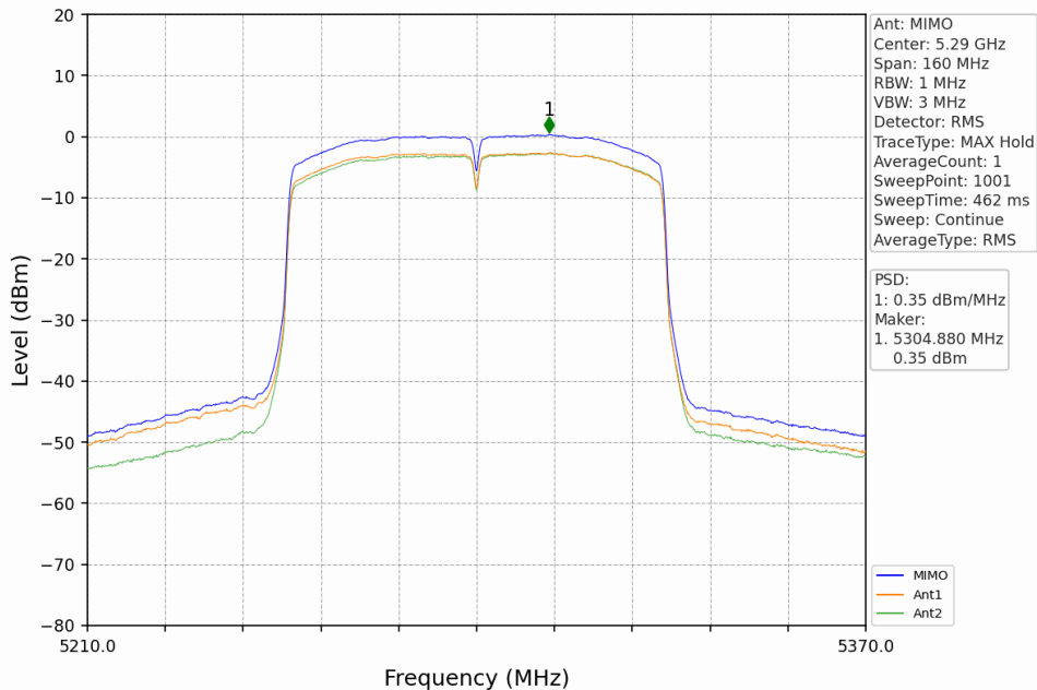
802.11ac(VHT80)_MCH_5290MHz_MIMO_NTNV
