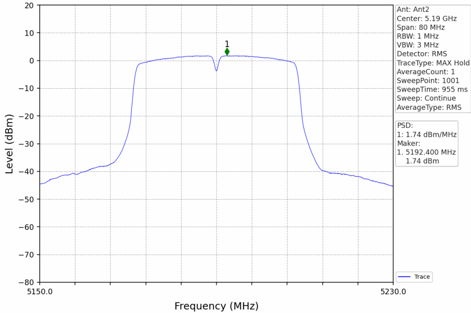
802.11ac(VHT40)_LCH_5190MHz_MIMO_NTNV
