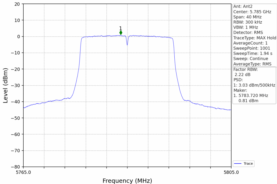
802.11ac(VHT20)_MCH_5785MHz_Ant2_NTNV
