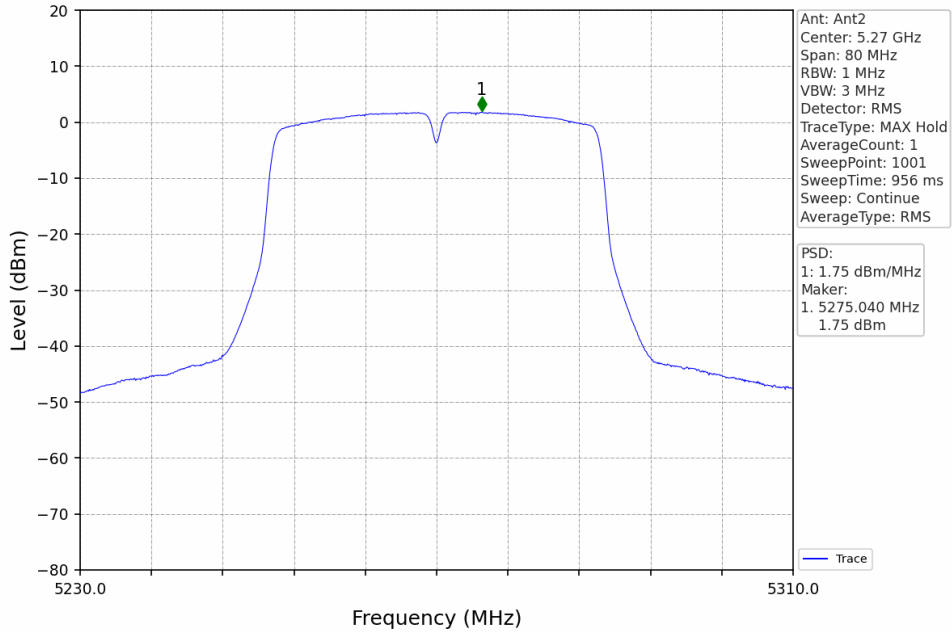
802.11ac(VHT40)_LCH_5270MHz_MIMO_NTNV
