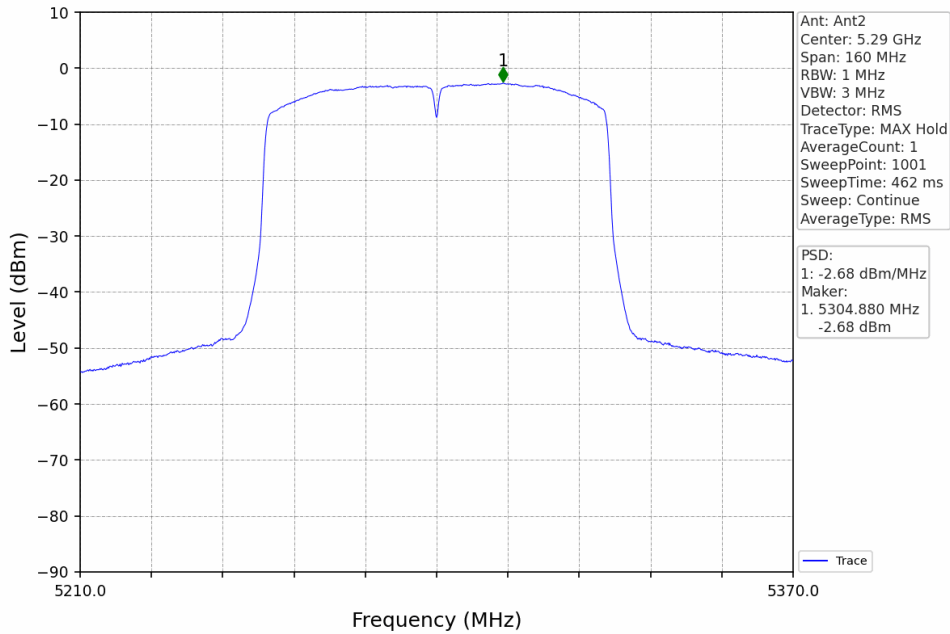
802.11ac(VHT80)_MCH_5290MHz_MIMO_NTNV
