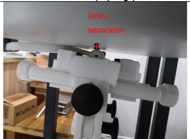
Head SAR (Left Edge)
