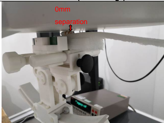
Head SAR (Right Edge)
