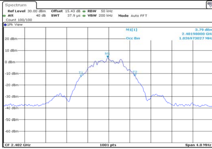
BLE_1M_Ant1_2402
