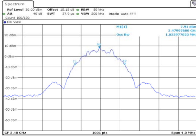
BLE_1M_Ant1_2480
